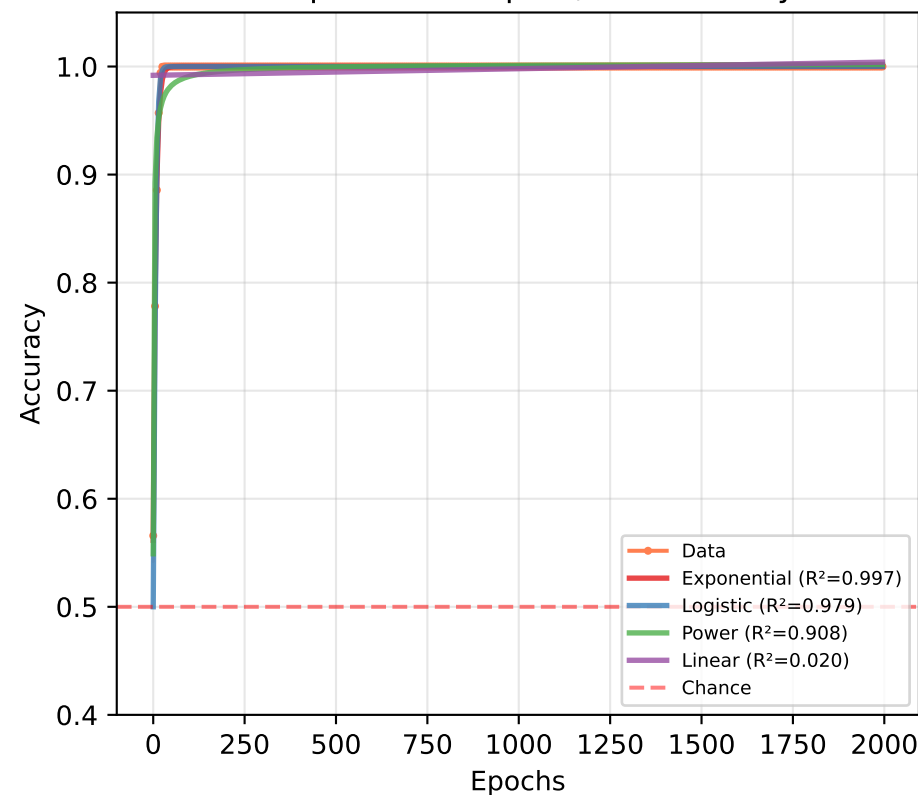
B: Parallel XORs (Non-Compositional) "Independent outputs, no hierarchy"
