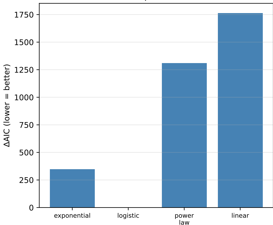
Model Comparison (Compositional)
