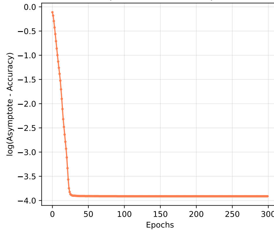
Log-Linear Plot (Exponential → linear slope)
