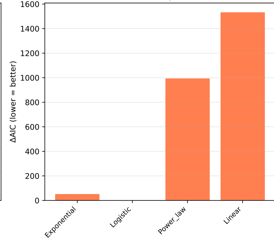
Model Comparison
