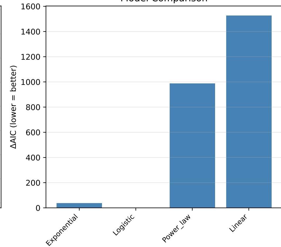
Model Comparison
