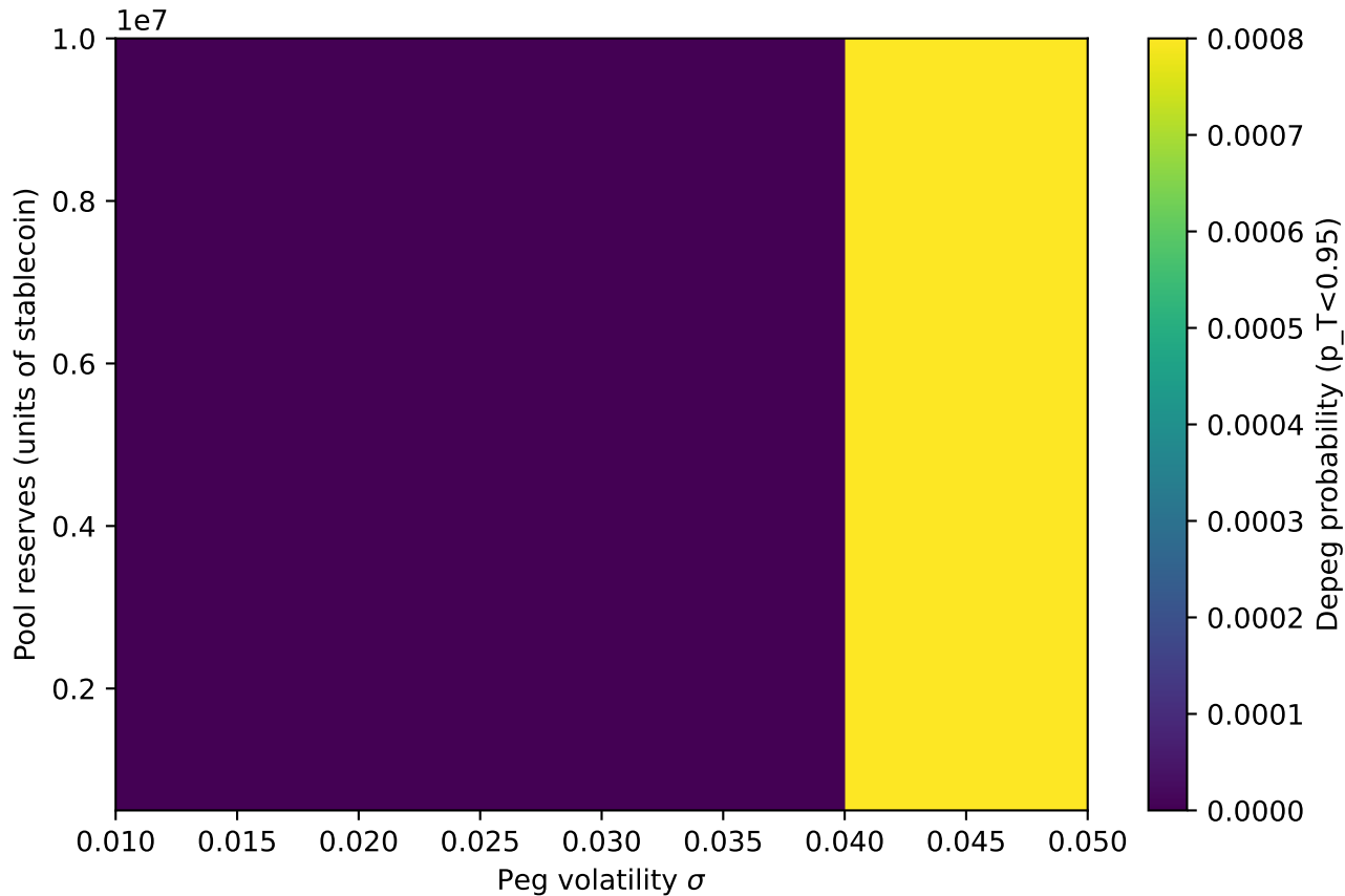
Depeg heatmap: \sigma \times reserves ( \kappa = 5.0 , trade=10\%)
