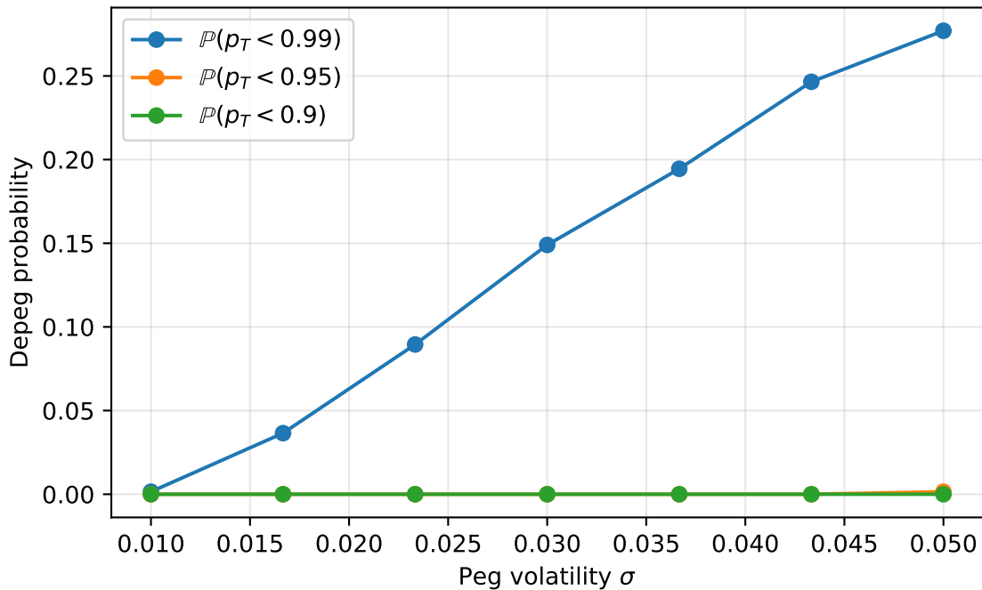
Depeg probability vs volatility \sigma (OU peg, \kappa = 5.0 )
