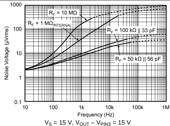
Figure 11. Output Noise Voltage vs Measurement Bandwidth
