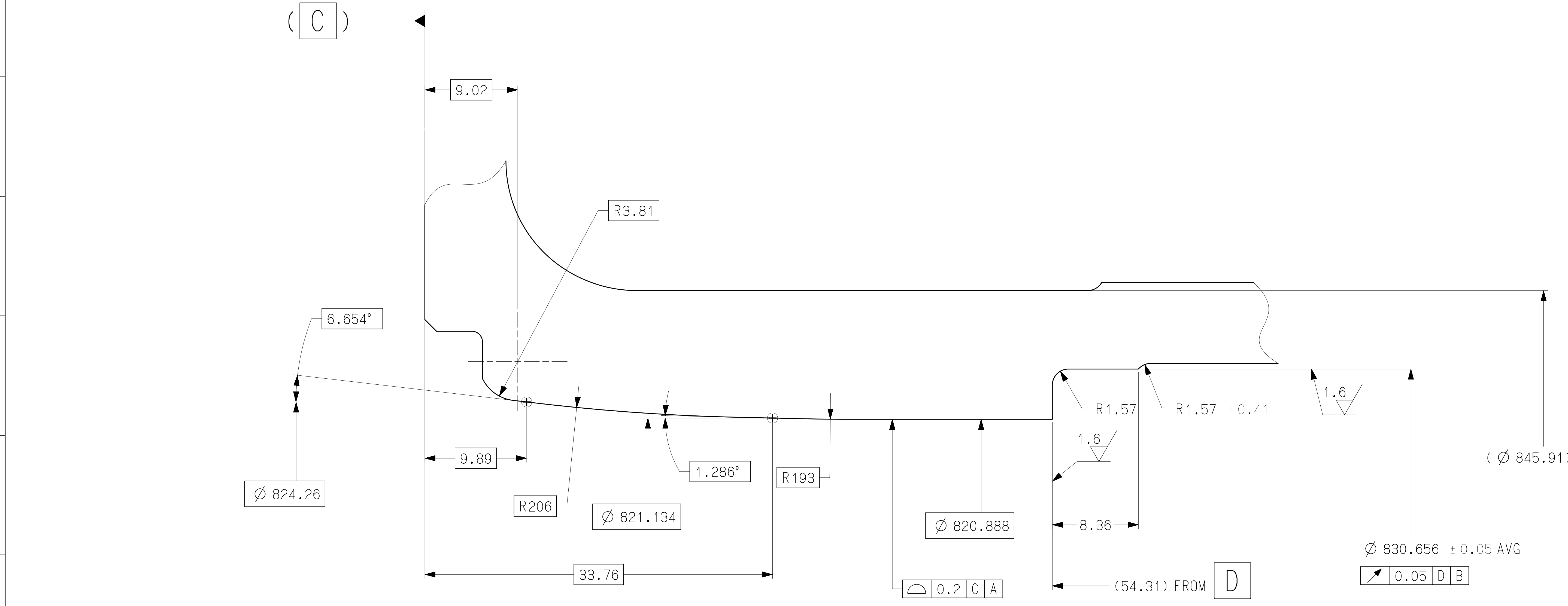
DETAIL BA (F8-2) SCALE 5:1
