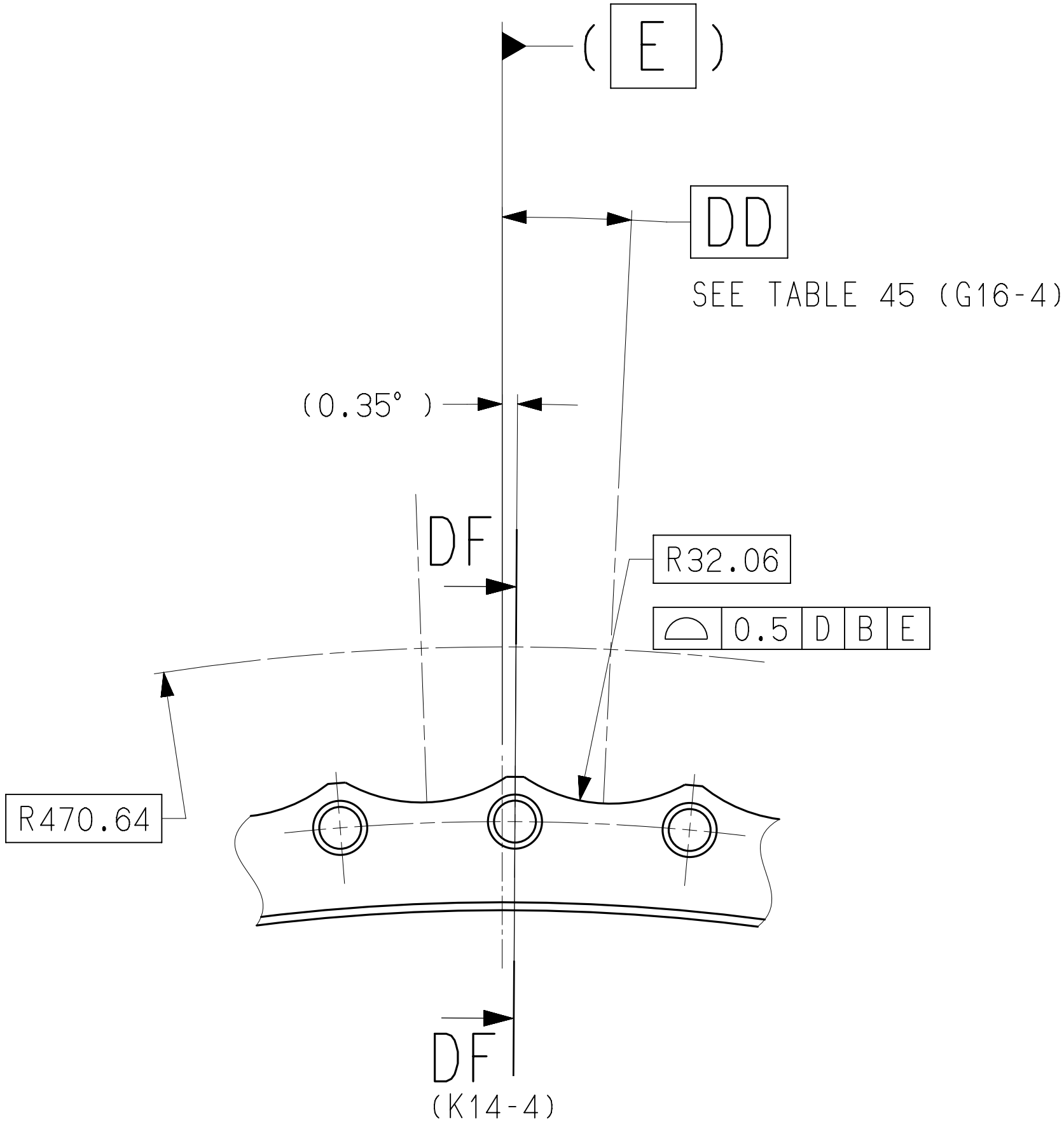
DETAIL DC (D4-4) SCALE 1:1 64 PLACES
