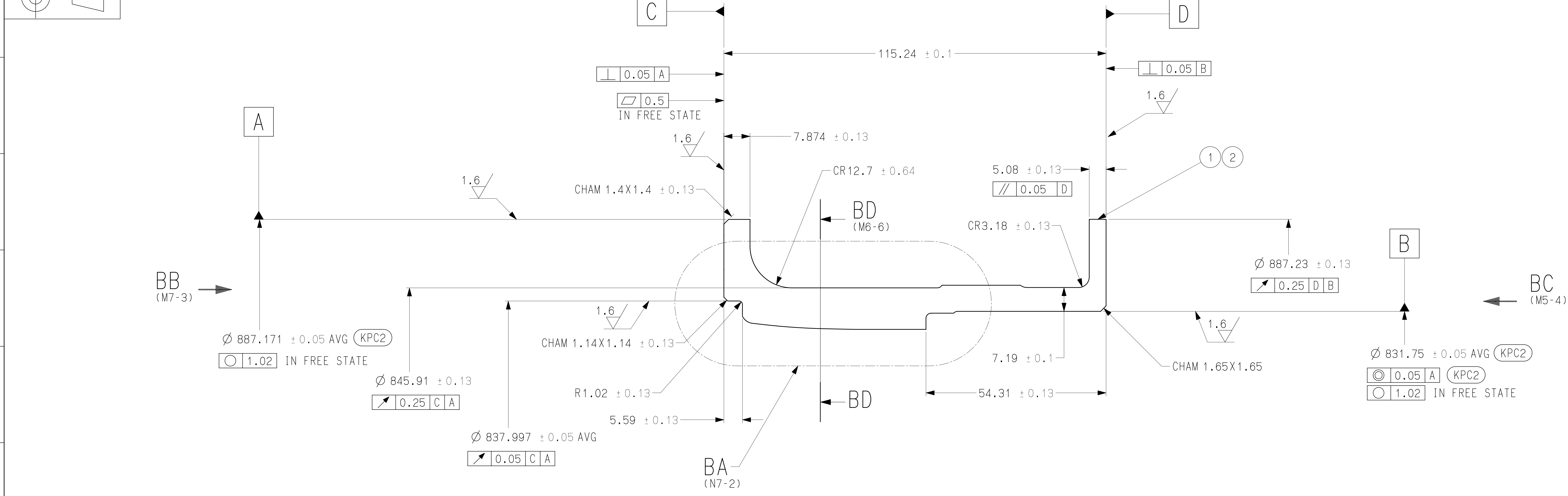
TYPICAL SECTION
