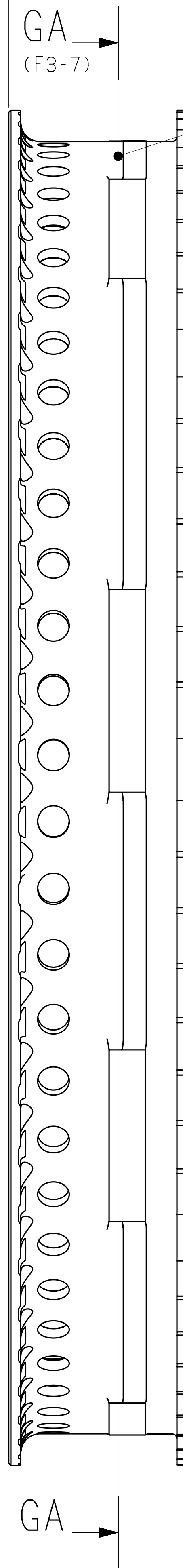
VIEW CG (G13-3) SCALE 1:2
