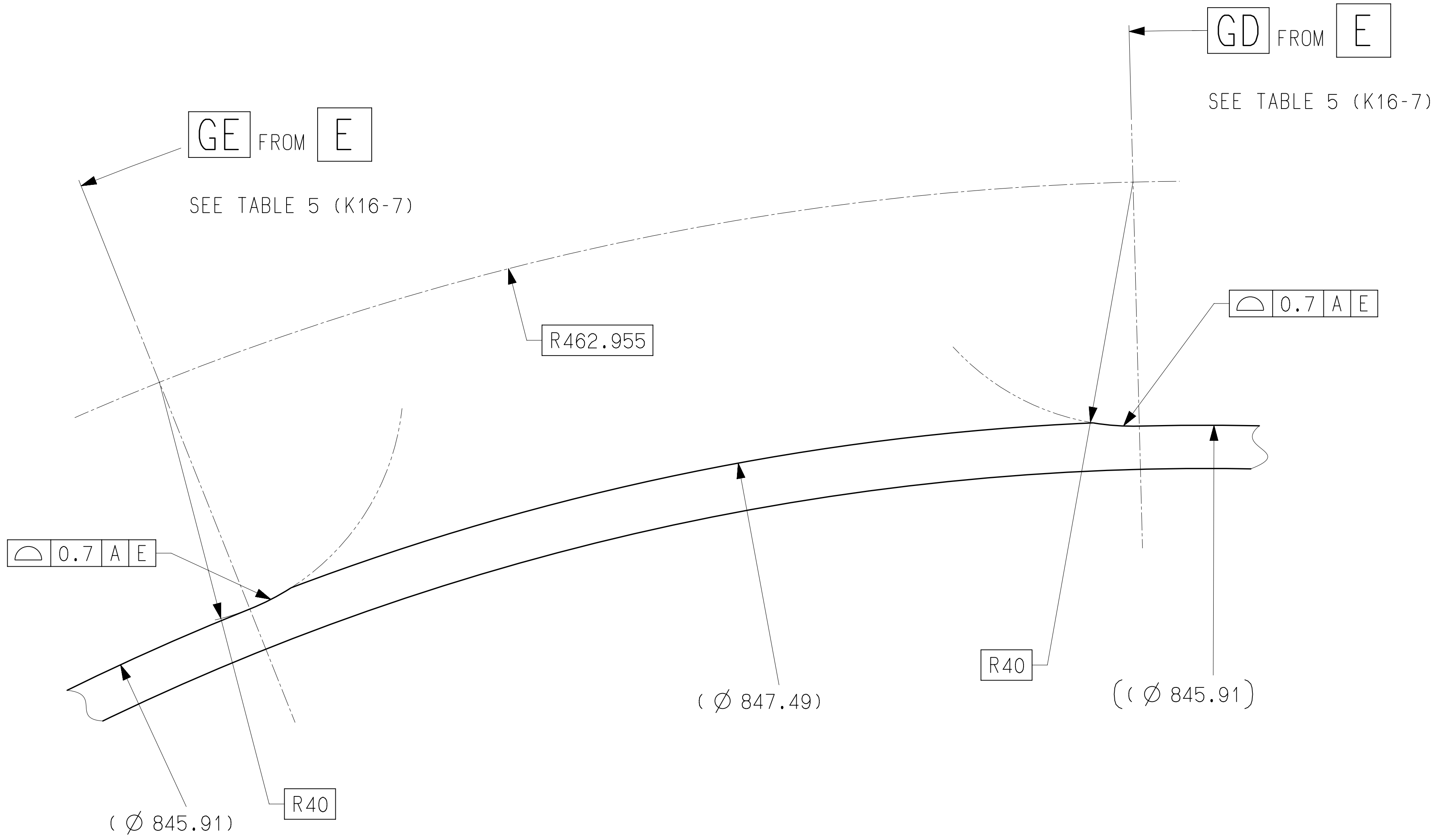
DETAIL GC (B2-7)
