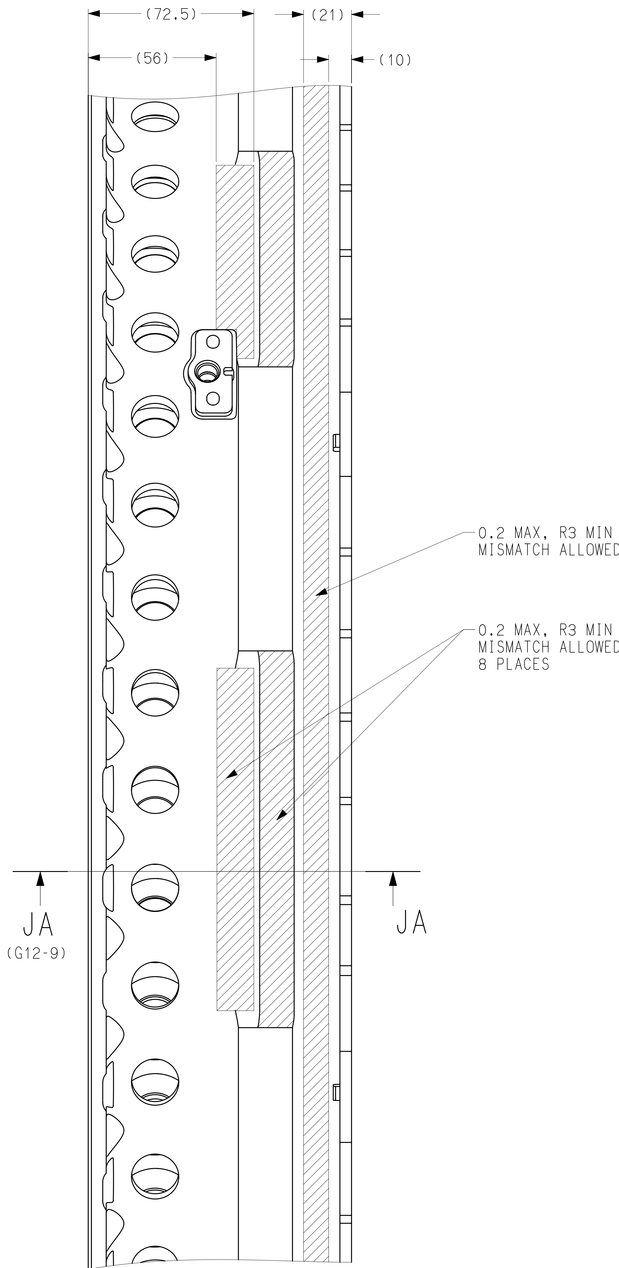
VIEW C J (C2-3) SCALE 1:1 ROTATED HORIZONTAL FOR CONVENIENCE
