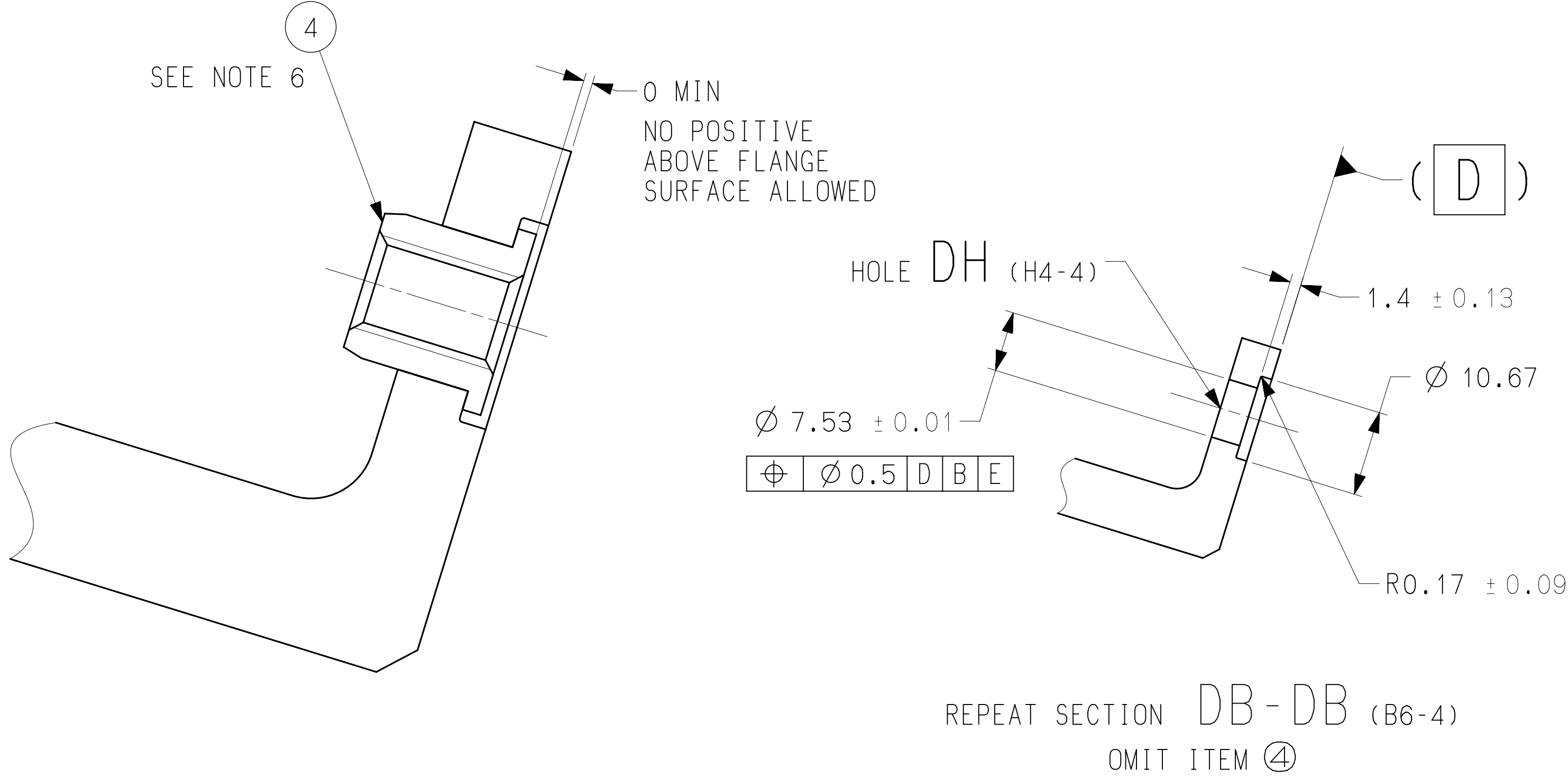
SECTION DB-DB (B6-4) SCALE 5:1 9 PLACES
