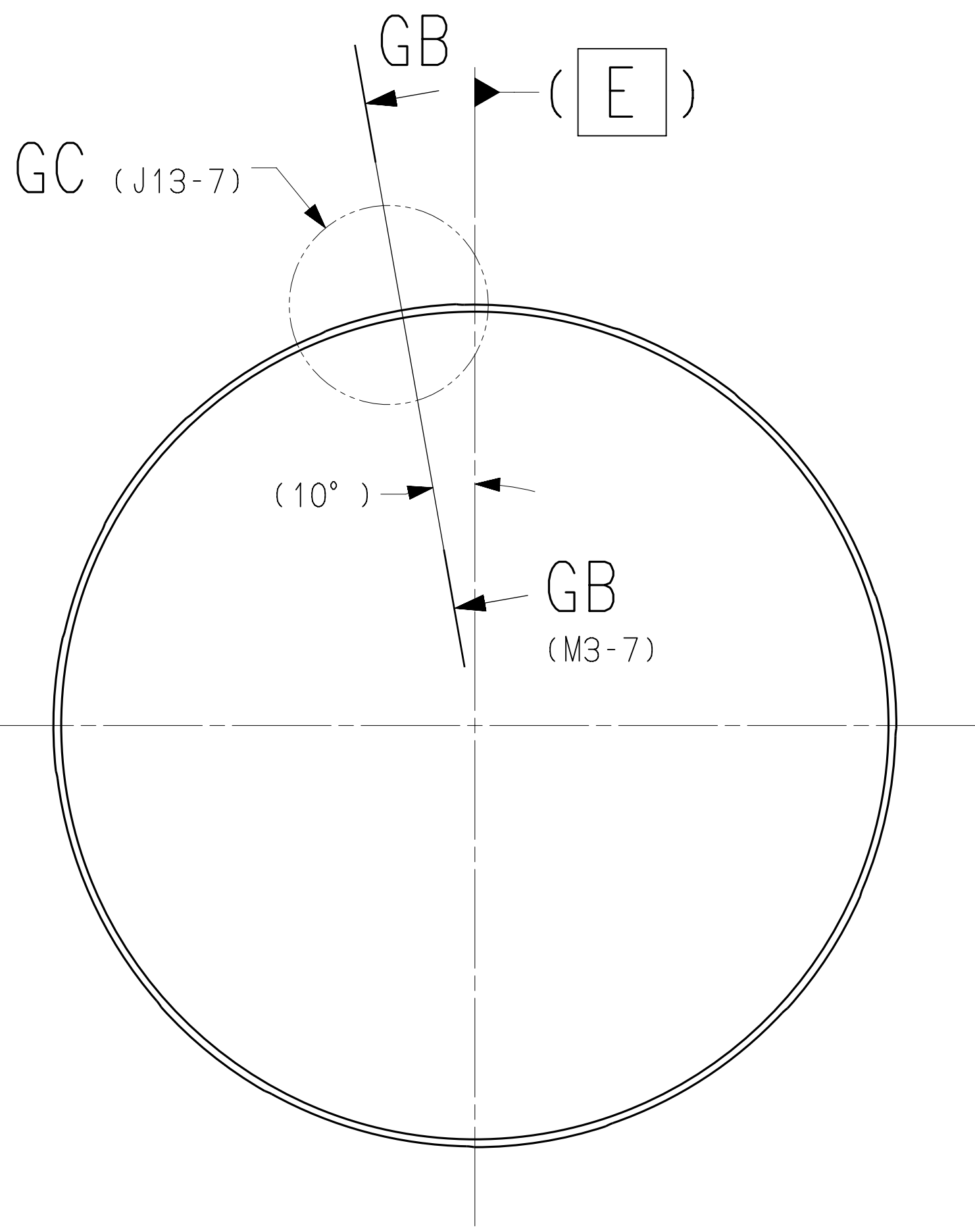
SECTION GA-GA (A8-7) SCALE 1:5
