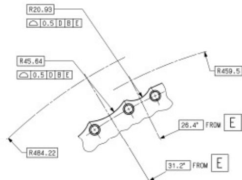
DETAIL DF (D5-4) SCALE 1:1
