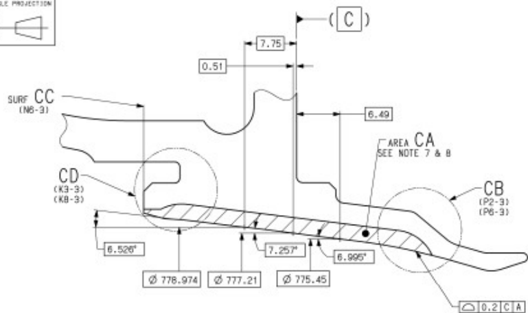
DETAIL BC (H19-2) SCALE 5:1
