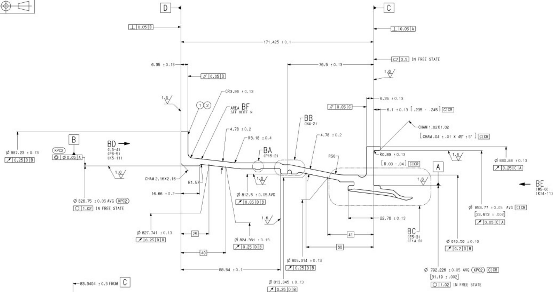
TYPICAL SECTION
