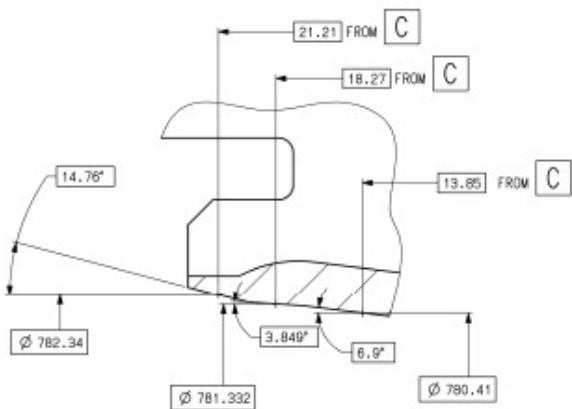
DETAIL CD (C2-3) SCALE 10:1
