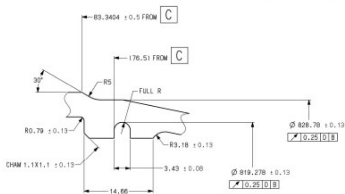
DETAIL BB (D10-2) SCALE 5:1
