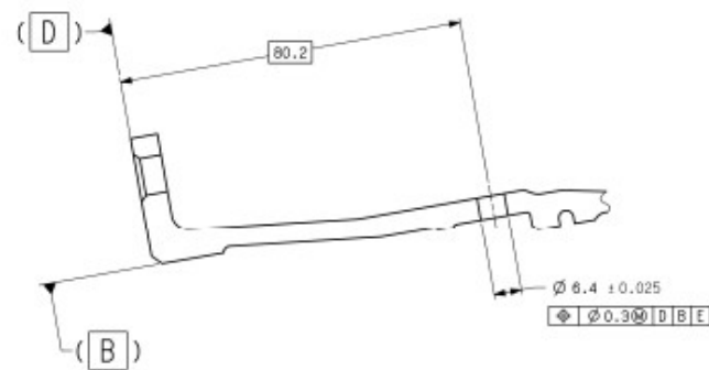
SECTION ED-ED (D5-5) 2 PLACES
