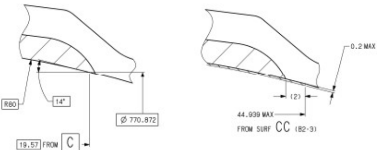
REPEAT DETAIL CB (C7-3) SCALE 10:1
