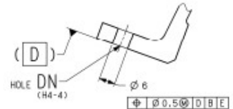
SECTION DE-DE (E1-4) 8 PLACES
