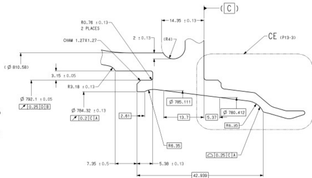
REPEAT DETAIL BC (H13-2) SCALE 5:1 BEFORE COATING
