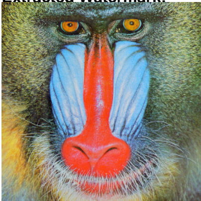
Extracted Watermark:
