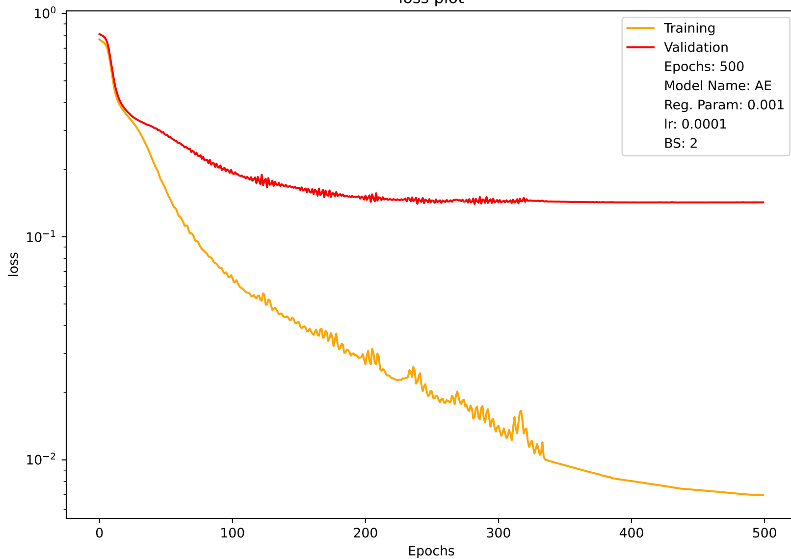
loss plot
