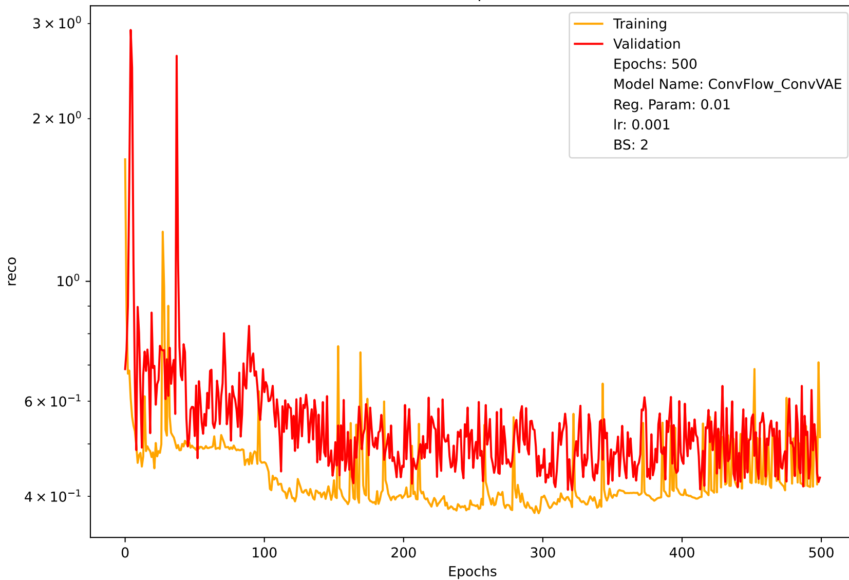
reco plot
