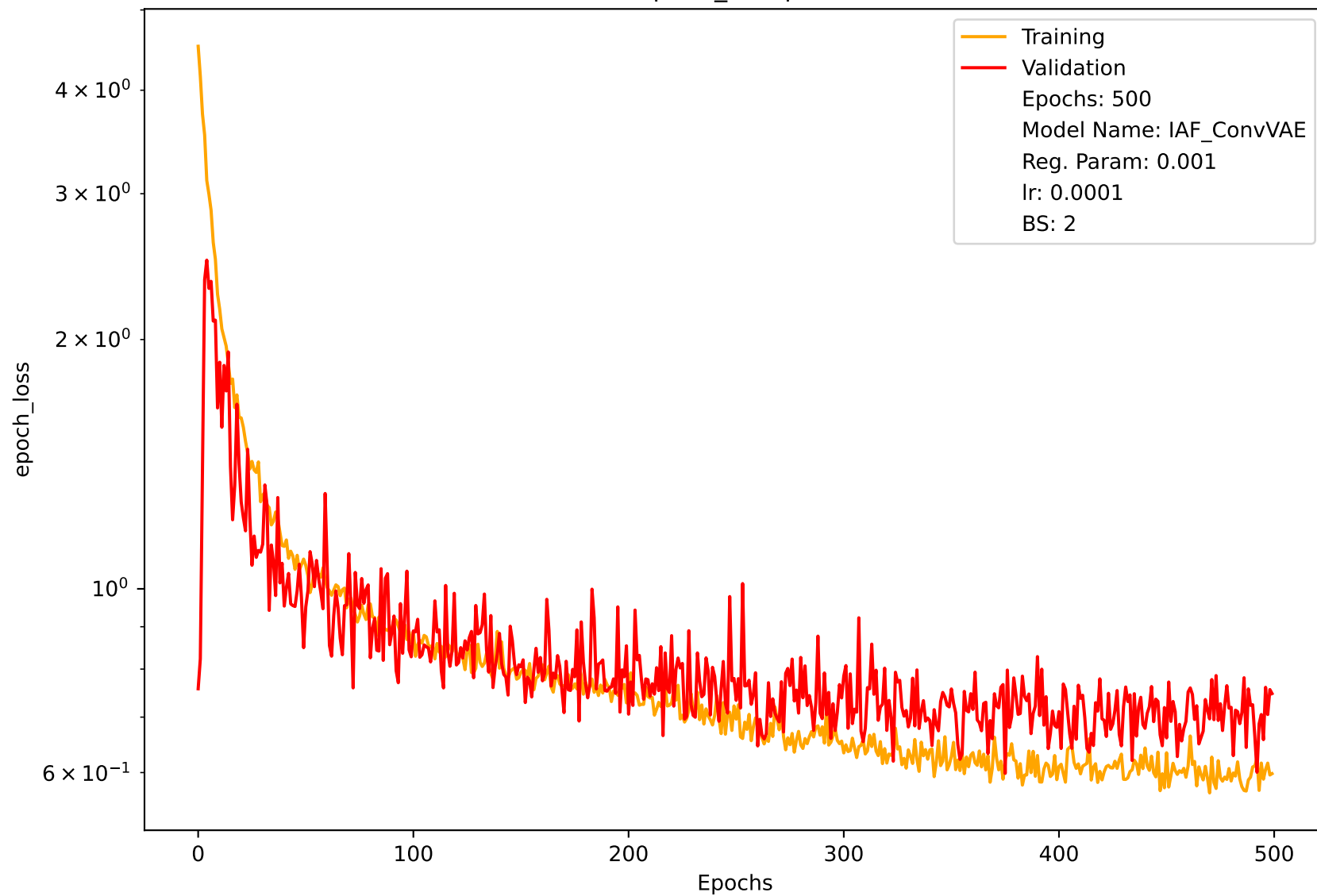
epoch_loss plot
