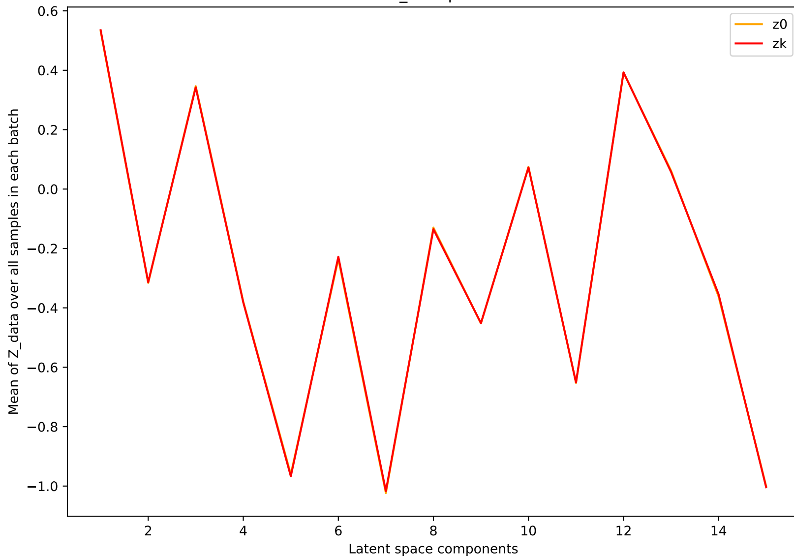
Z_data plot
