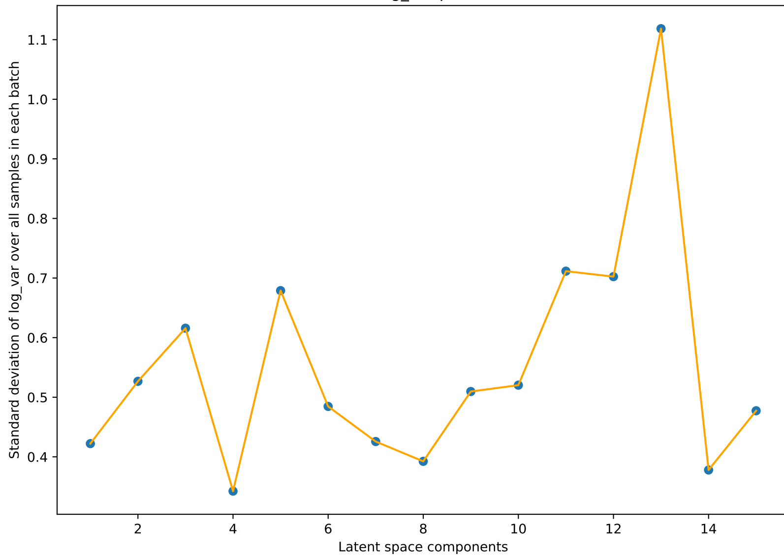
log_var plot
