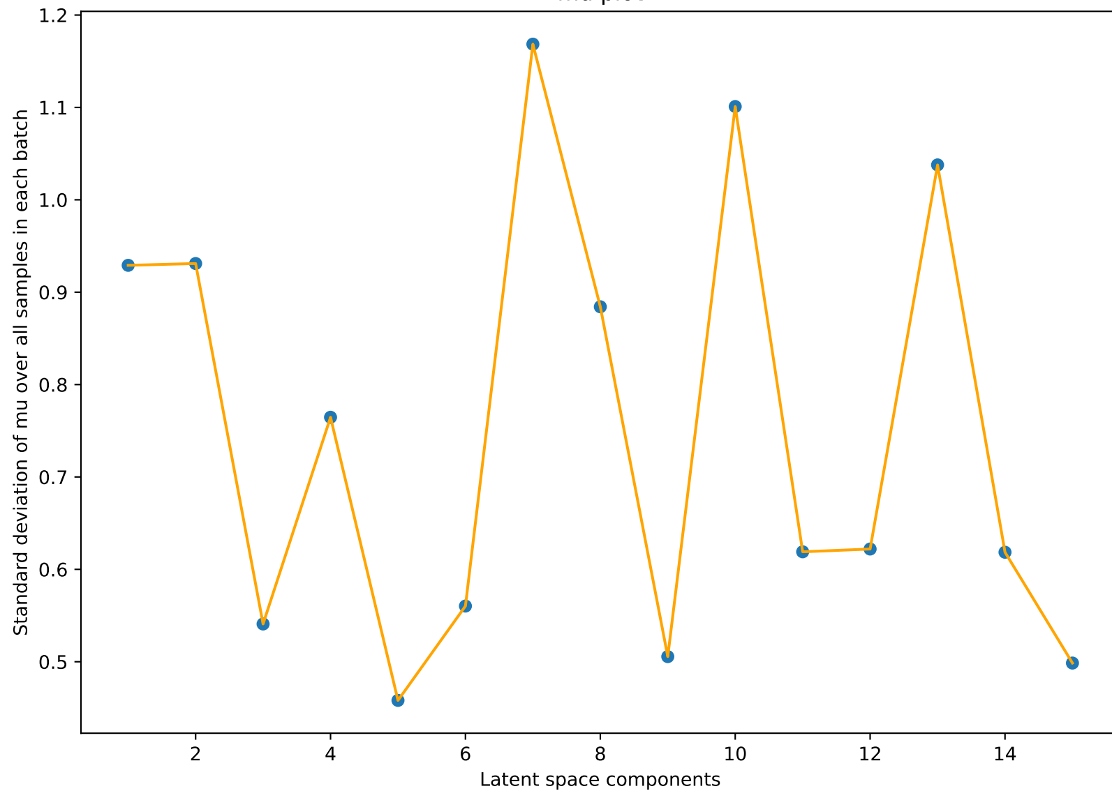
mu plot
