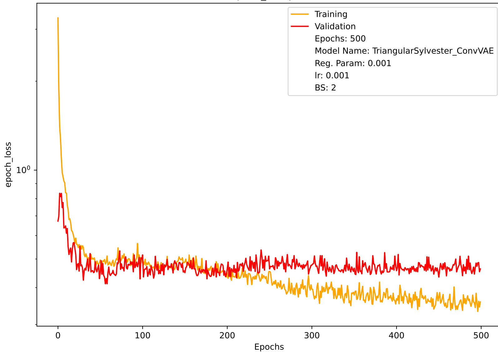
epoch_loss plot
