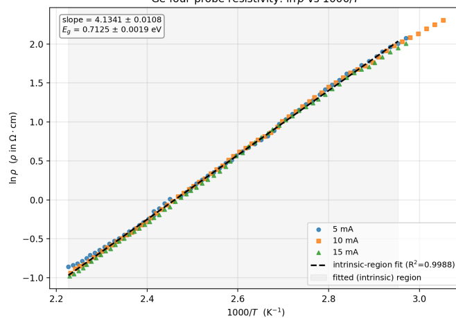
Ge four-probe resistivity: \ln \rho vs 1000/T
