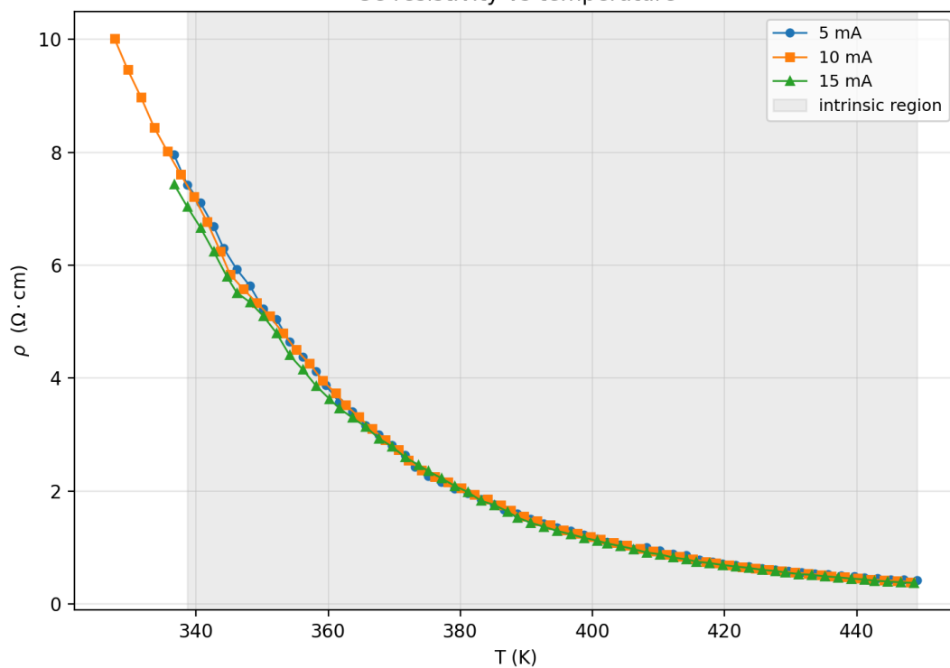
Ge resistivity vs temperature
