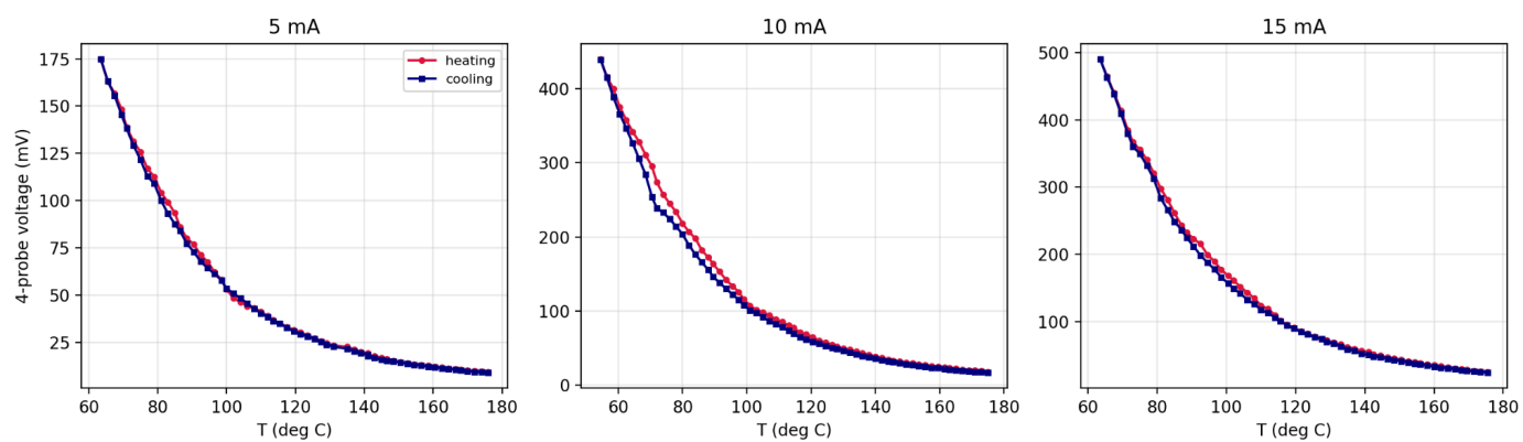
Heating vs. cooling repeatability check
