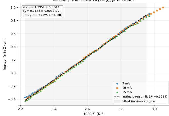
Ge four-probe resistivity: \log_{10} \rho vs 1000/T
