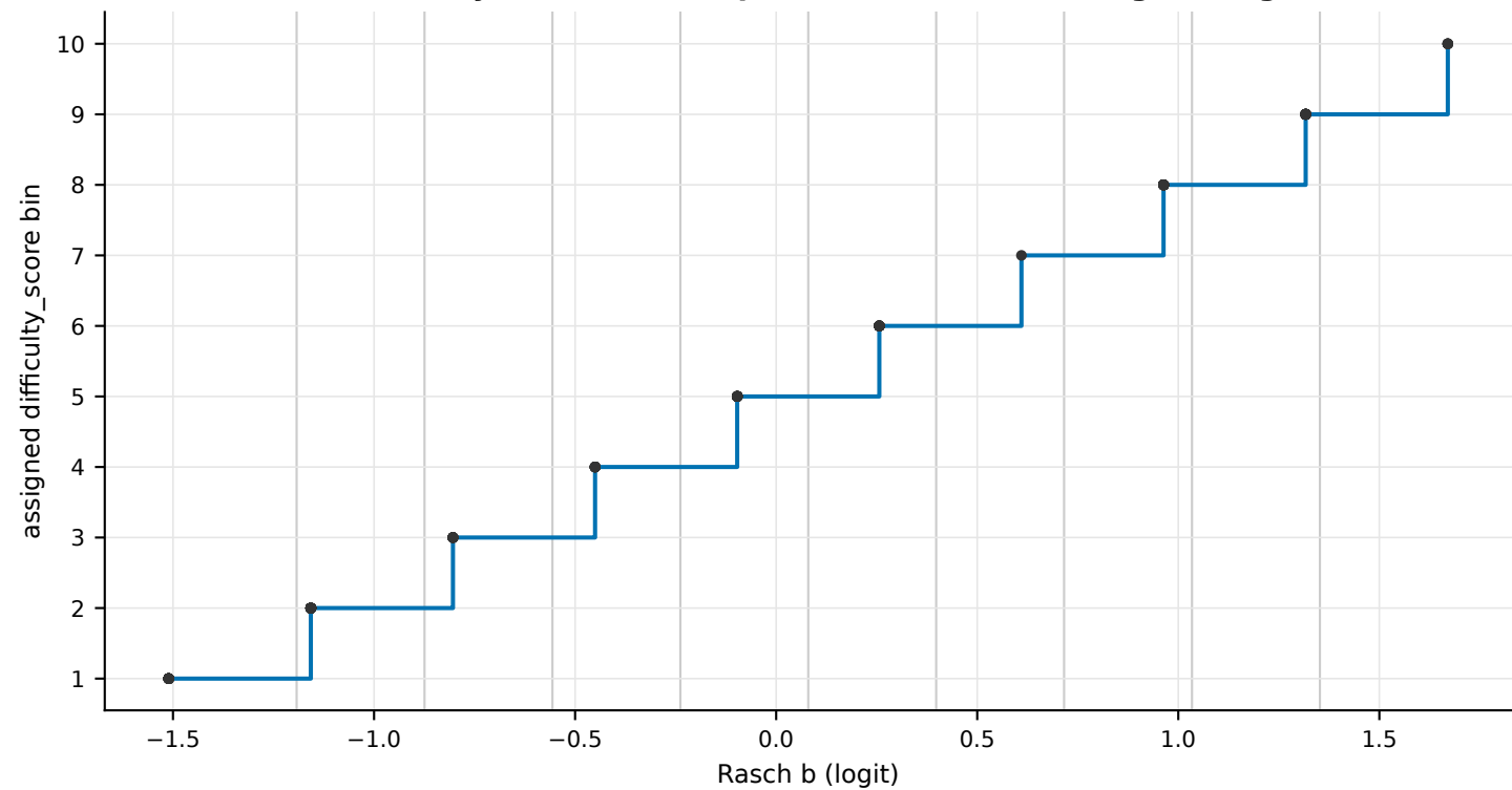
b → difficulty bin (10 bins, equal-width over the b range, 9 edges)
