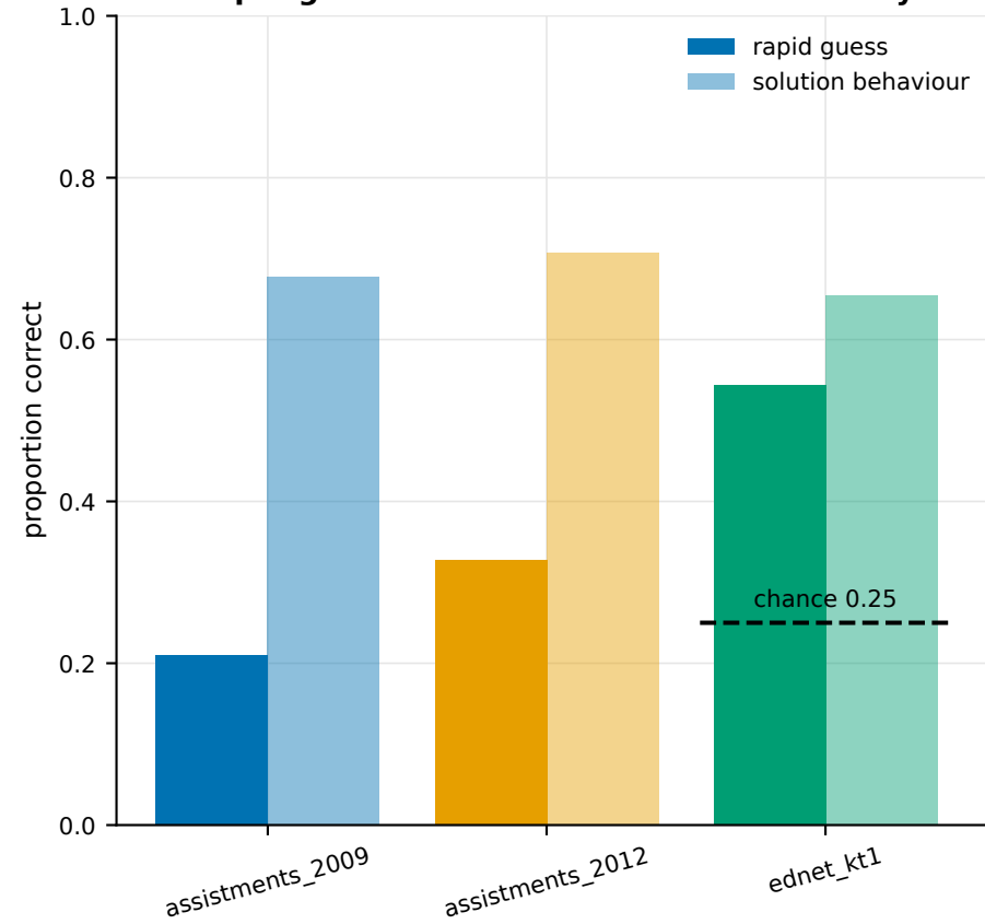
Rapid-guess vs solution behaviour accuracy
