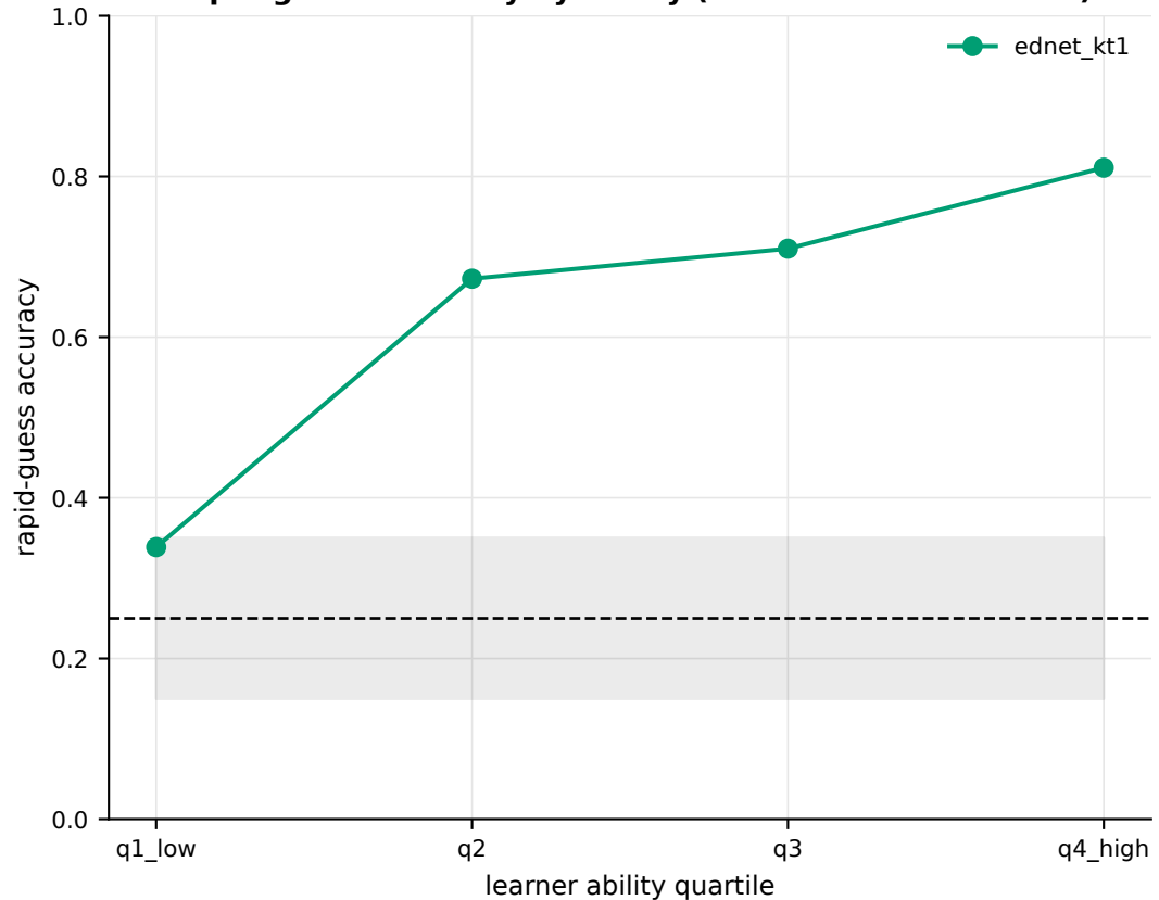
Rapid-guess accuracy by ability (shaded: chance \pm 0.10 )
