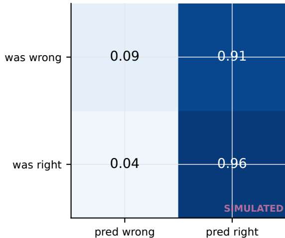
sim-V0 lightgbm
