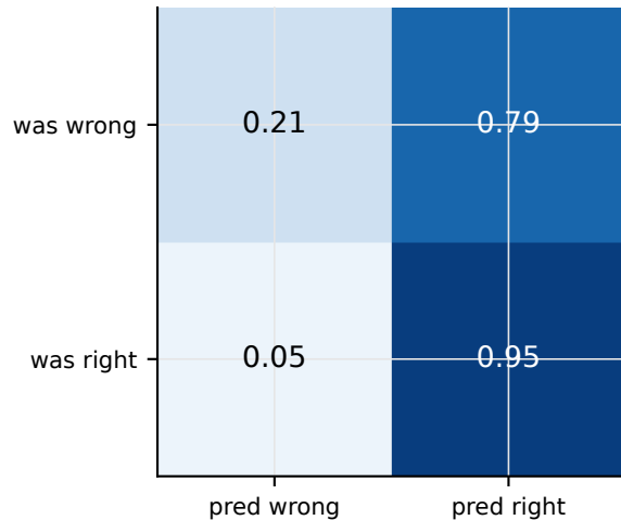
assistments_2012 lightgbm
