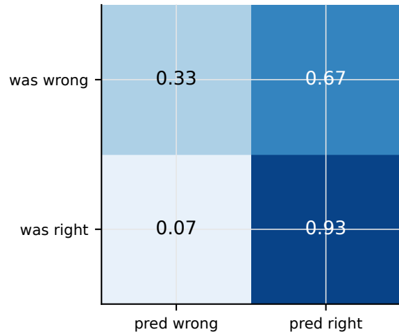
assistments_2009 lightgbm
