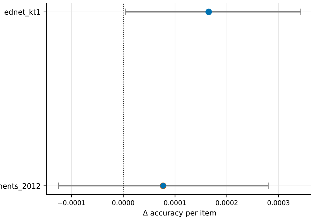
accuracy slope (the fatigue claim)
