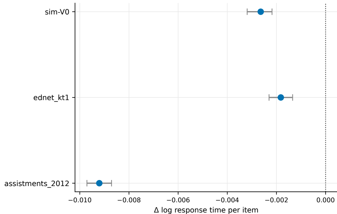
speed slope (the surviving observable)
