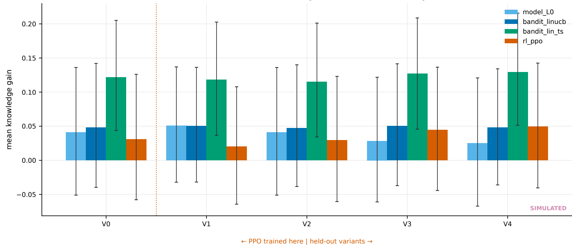
Trained on V0, evaluated on every variant — the credibility check
