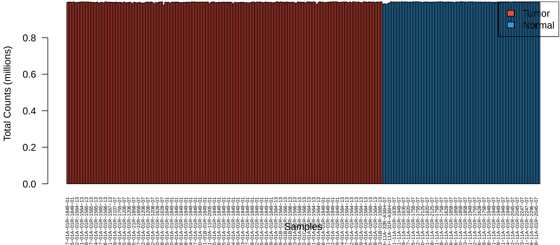
Library Sizes per Sample
