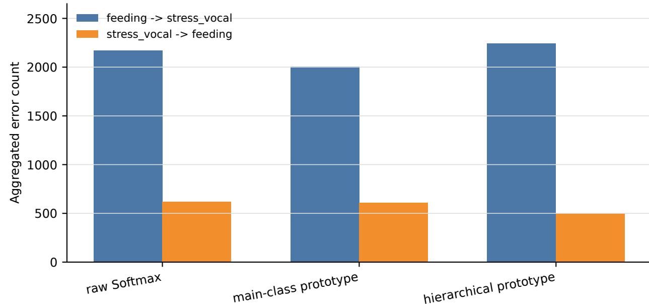
Feeding/Stress confusion under ALL_NOISY simulated additive noise
