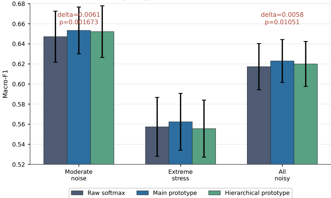
Main-class prototype is steadier under simulated noise
