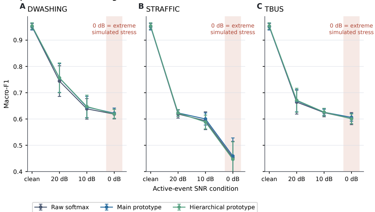
Figure 6 | Active-event SNR degradation under DEMAND simulated noise
