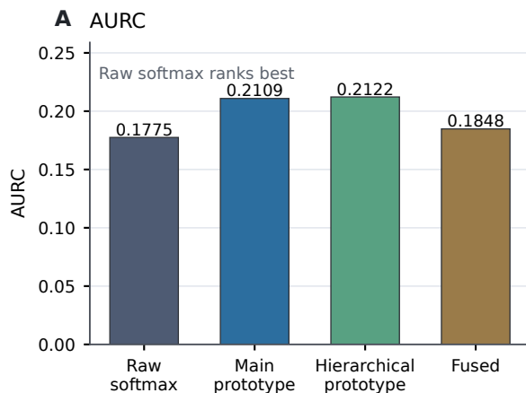
Figure 8 | Selective prediction under ALL_NOISY
