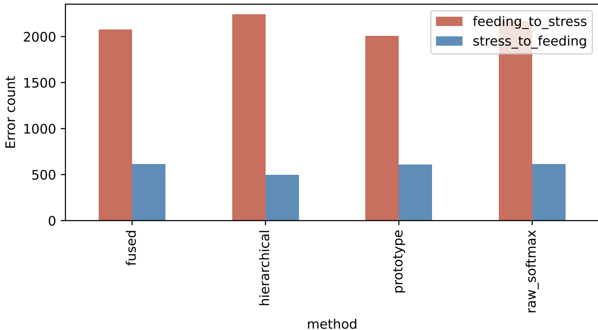
Feeding/Stress Confusion under ALL_NOISY
