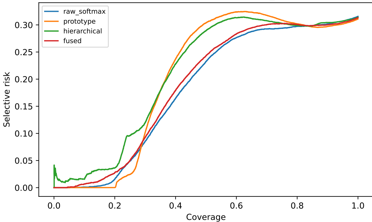
Risk-Coverage Curves under ALL_NOISY
