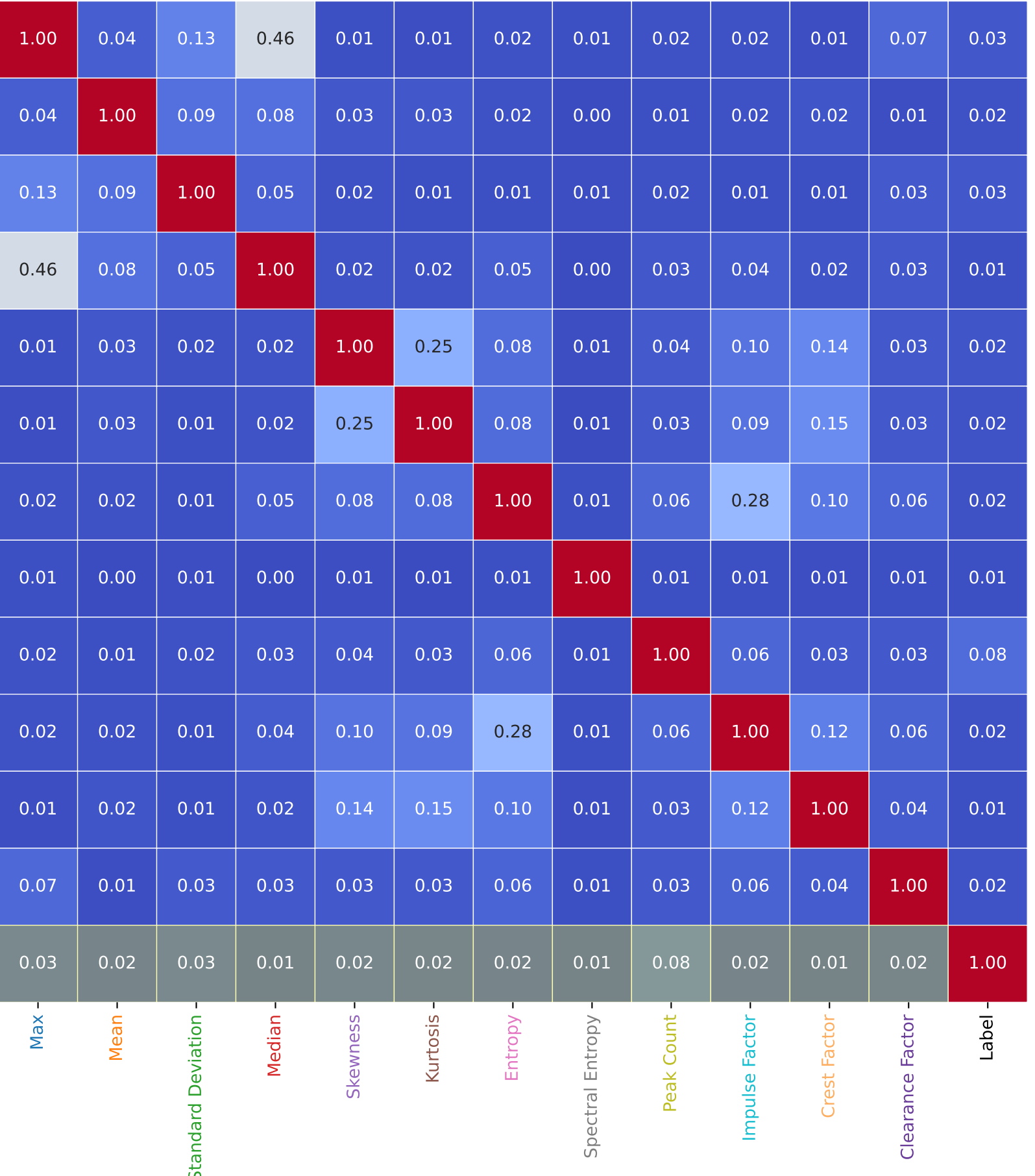
Normalized Mutual Information Matrix of Features and Label)
