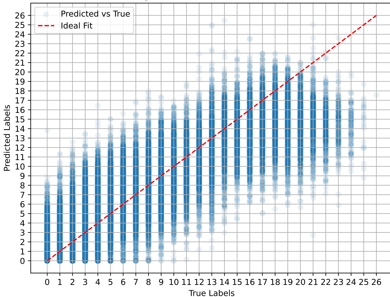
LinearRegression: Predictions Across All Folds
