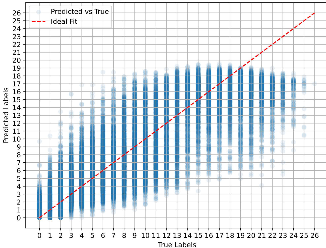
MLPRegressor: Predictions Across All Folds
