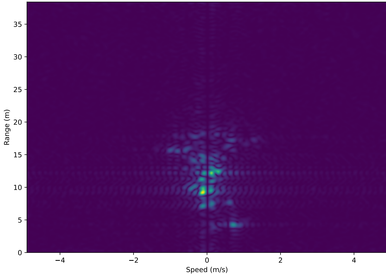
Radar Doppler Map - Amplitude (22 people)
