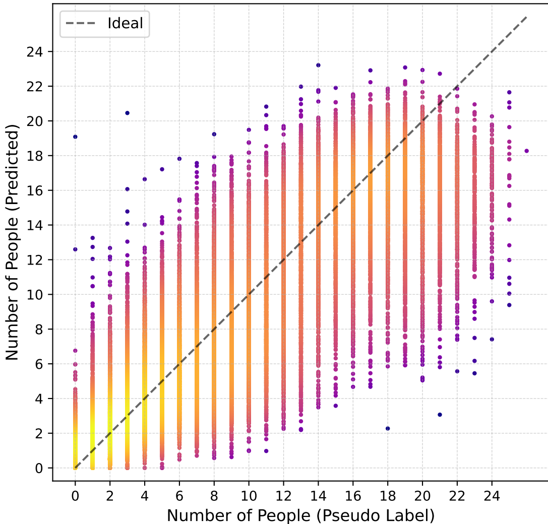
SVR: Predictions vs Pseudo Label
