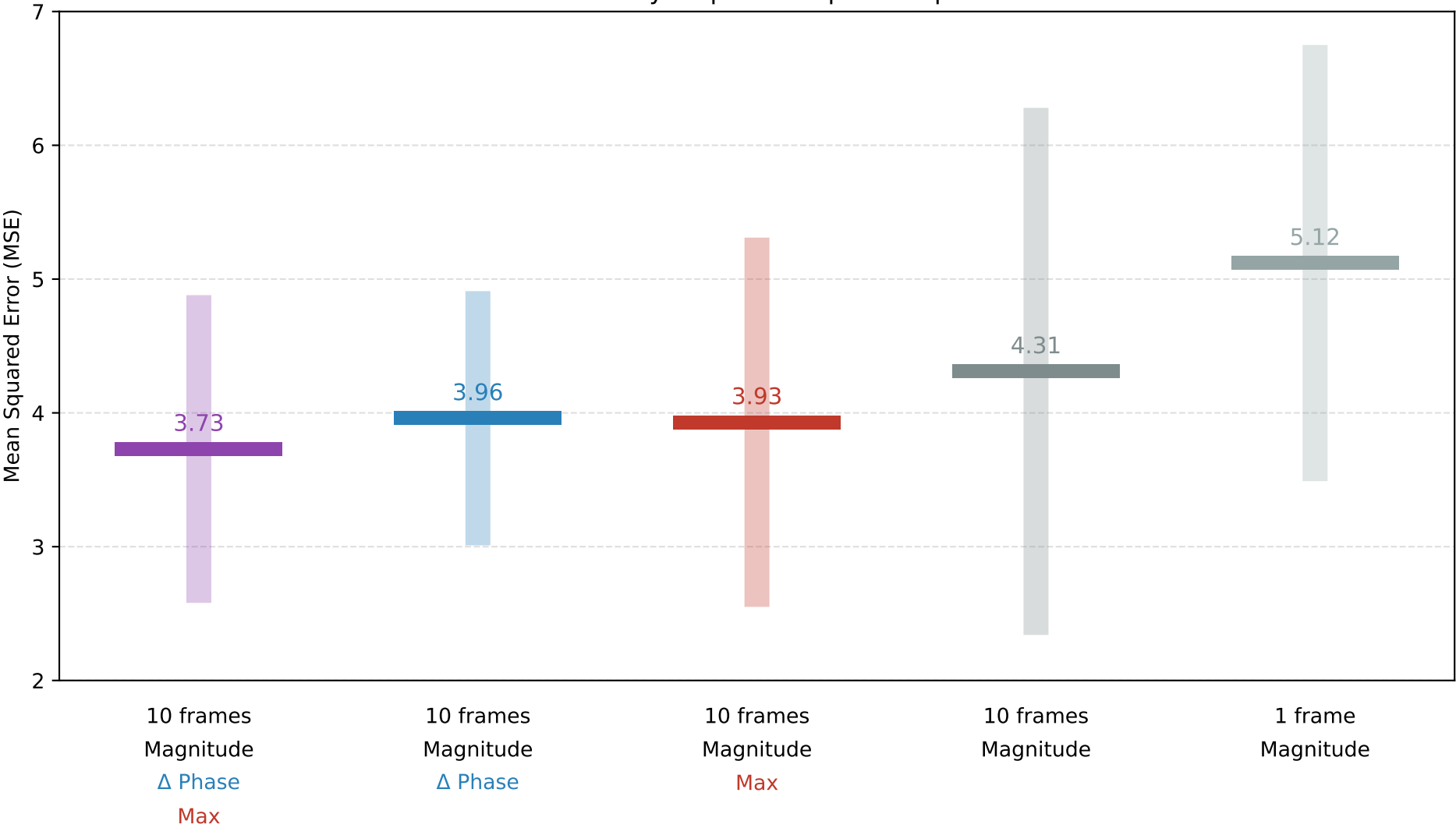
Ablation Study: Impact of Input Composition
