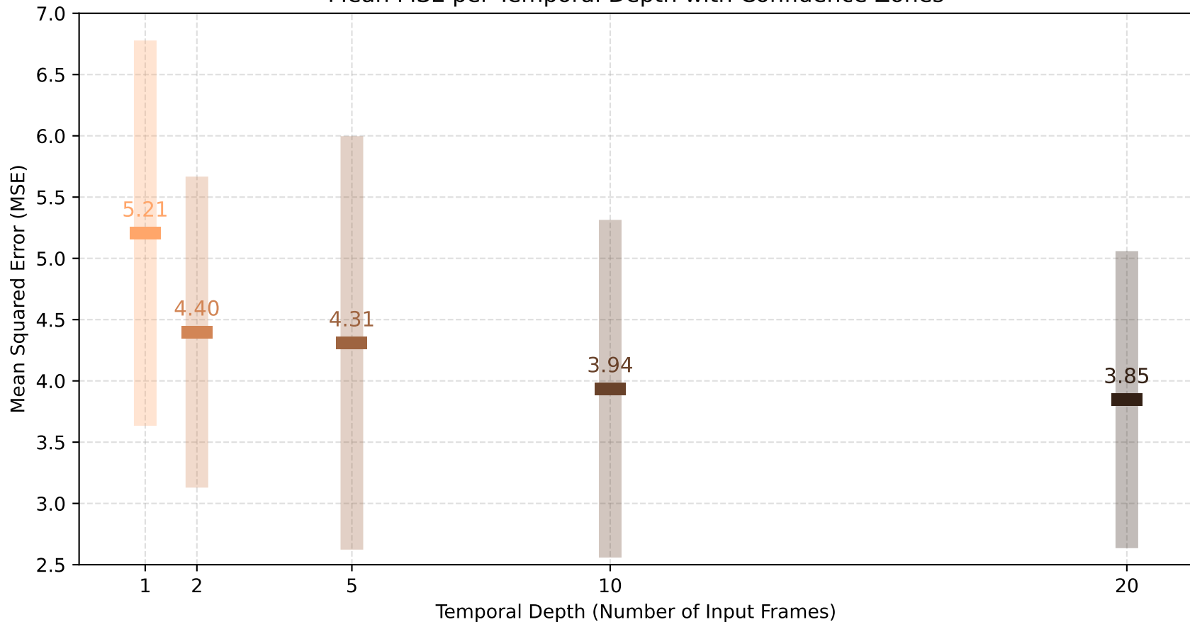
Mean MSE per Temporal Depth with Confidence Zones
