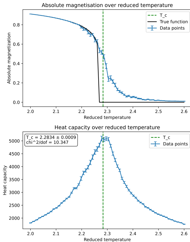
FIG. 3. Plots of average absolute magnetisation and heat capacity over the reduced temperature showing also the true function for magnetisation given by Eq. (8) and the calculated value of T_c .
