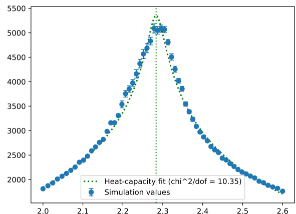
FIG. 2. Calculated heat capacity results and a fit through using function in Eq. (12) with found value of critical temperature being T_c = 2.2834 \pm 0.0009 .
