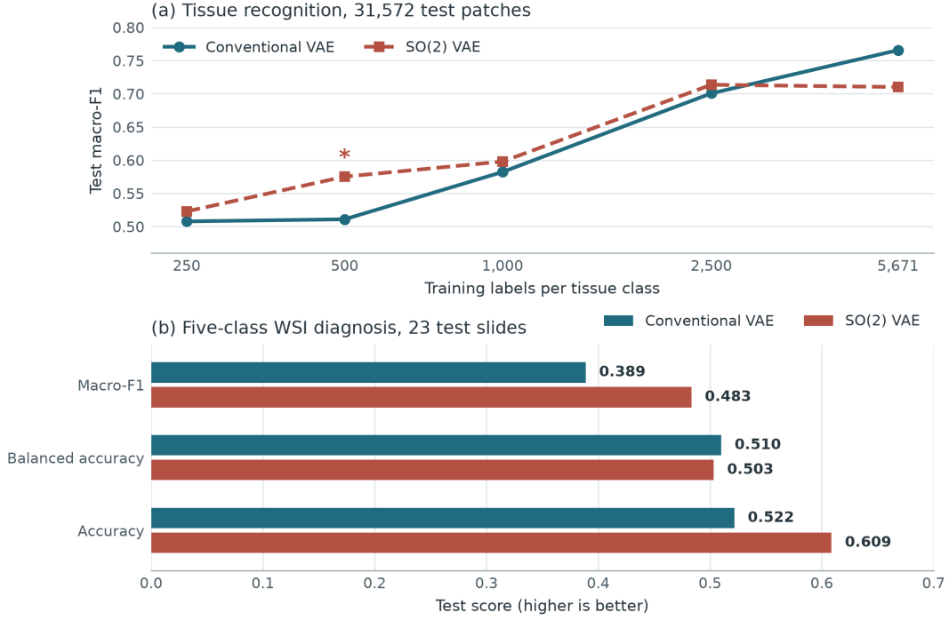
Figure 10: Frozen-representation classification results. (a) Tissue macro-F1 on 31,572 test patches under nested class-balanced training budgets; the asterisk marks the 500-label contrast whose simultaneous 95% difference interval excludes zero. (b) Five-class diagnosis on 23 test WSIs. The paired WSI macro-F1 interval includes zero.
