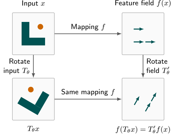
Figure 1: Rotation equivariance as a transformation law. The two paths from x to the lower-right field agree for an equivariant mapping f . The input rotation T_\theta acts on the image; the corresponding output action T'_\theta also rotates vector components when the output contains vector fields. Shapes and arrows are schematic rather than measured VAE features.
