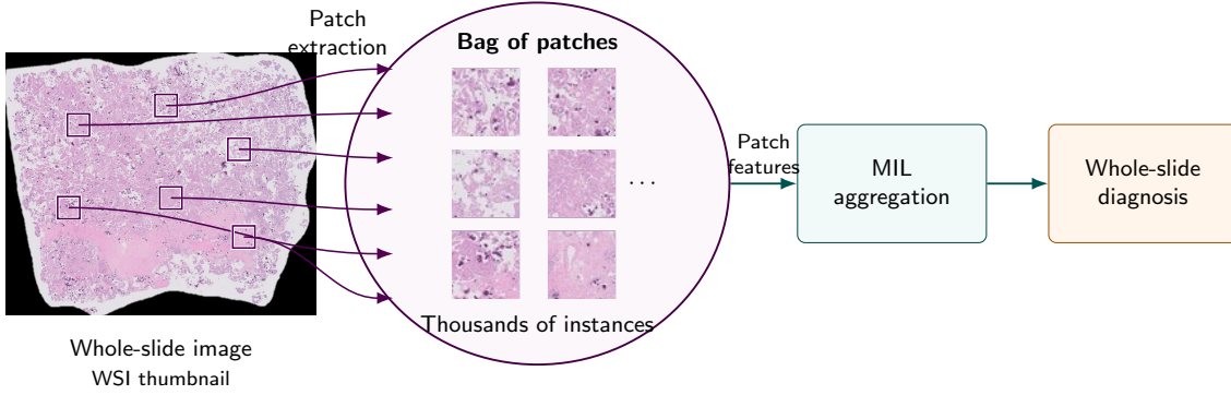
Figure 2: Multiple-instance learning for WSI diagnosis. Many patches extracted from one slide form a bag. Their encoded features are aggregated to predict one whole-slide diagnosis. The six thumbnail regions illustrate the slide-to-bag construction; the ellipsis represents the many remaining instances. In this study, patch features are obtained from frozen VAE posterior means, and supervision is provided by the WSI diagnosis label.
