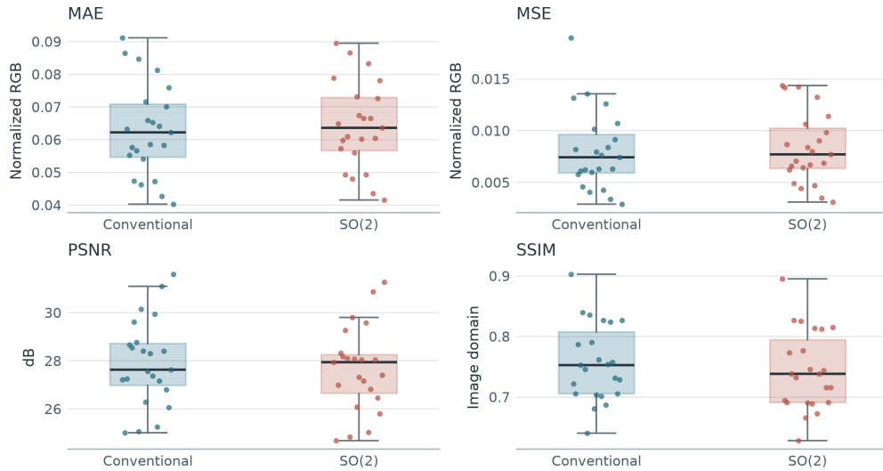
Figure 9: Reconstruction metric distributions across 23 test WSIs. Each point is one WSI-level mean; boxes summarize those 23 means for each frozen VAE. They are descriptive distributions, not confidence intervals. MAE and MSE use normalized RGB; PSNR and SSIM use image-domain values.
