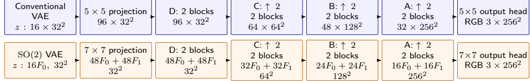
Figure 7: Layer-level architecture of the two frozen VAEs. The residual building blocks are detailed in Figure 6. Each stage A–D contains two residual blocks; stage-changing blocks additionally resample both branches and project the skip branch. A conventional hidden width is a channel count; in the SO(2) model, nF_0 + nF_1 means n scalar fields and n two-component vector fields. Posterior mean and log-variance use separate heads; training samples \mathbf{z} , whereas downstream classifiers use \boldsymbol{\mu} . The conventional stem uses a 7 \times 7 kernel and its other convolutions use 5 \times 5 kernels; the SO(2) stem uses a 9 \times 9 steerable kernel and its other convolutions use 7 \times 7 kernels. See Section 3.6.1 for the kernel-support rationale and learned-parameter comparison.
