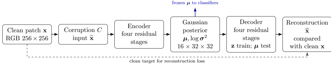
Figure 5: Shared denoising VAE workflow. Both models have the same input, posterior shape and encoder–decoder resolution schedule. They differ in the type of convolution and the accompanying field normalization and gates. Training reconstructs the clean patch from a possibly corrupted input; classification uses only the frozen posterior mean. The dashed rectangular path supplies the clean input as the reconstruction target.
