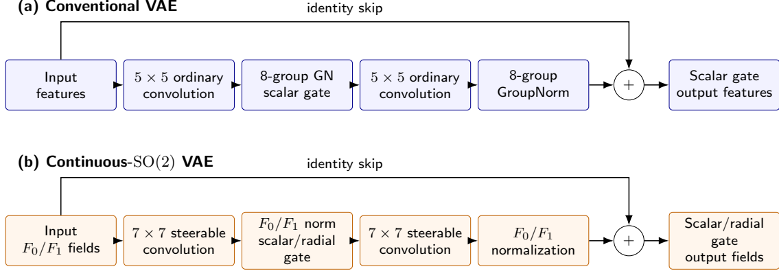
Figure 6: Same-resolution residual blocks used by the conventional and continuous-SO(2) VAEs. Each main branch contains two learned convolutions; normalization and a gate follow the first convolution, while the second is followed by normalization. The identity skip is added before the output gate. At encoder stage transitions, both branches are downsampled separately with a fixed 5 \times 5 binomial filter: on the main branch after the first gate and on the skip branch before its learned projection and normalization. At decoder transitions, both branches are bilinearly upsampled before their first learned convolution; the skip branch again uses a projection and normalization. The F_0/F_1 field types and gate equations are defined in the surrounding text. The 7 \times 7 steerable support provides fuller sampling of the selected radial and angular basis; Section 3.6.1 gives the rationale and learned-parameter comparison.
