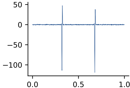
simulation, Y = 1
