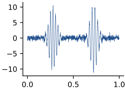
simulation, Y = 1
