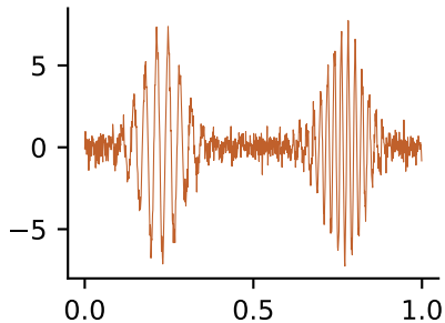
simulation, Y = 0
