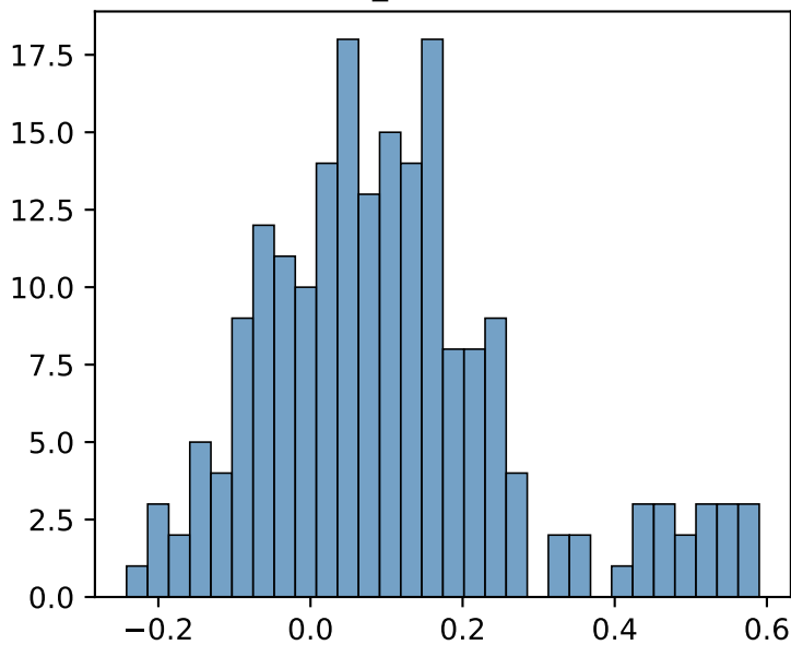
Flatness_std distribution
