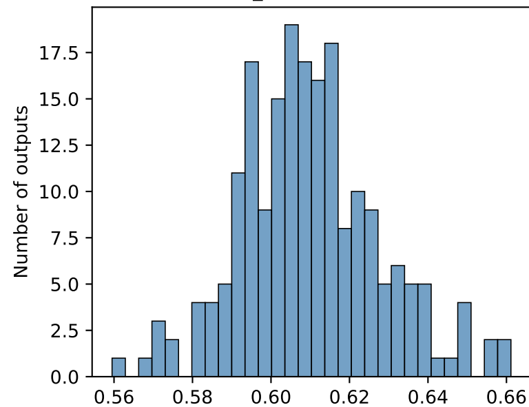
Flux_mean distribution
