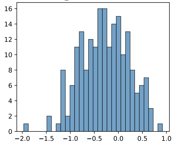
Flatness_skewness distribution
