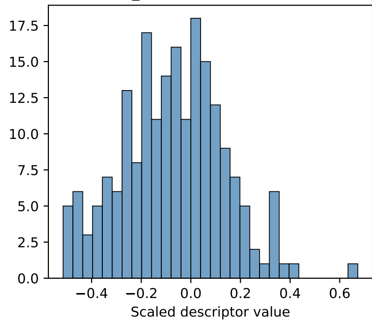
Flux_skewness distribution
