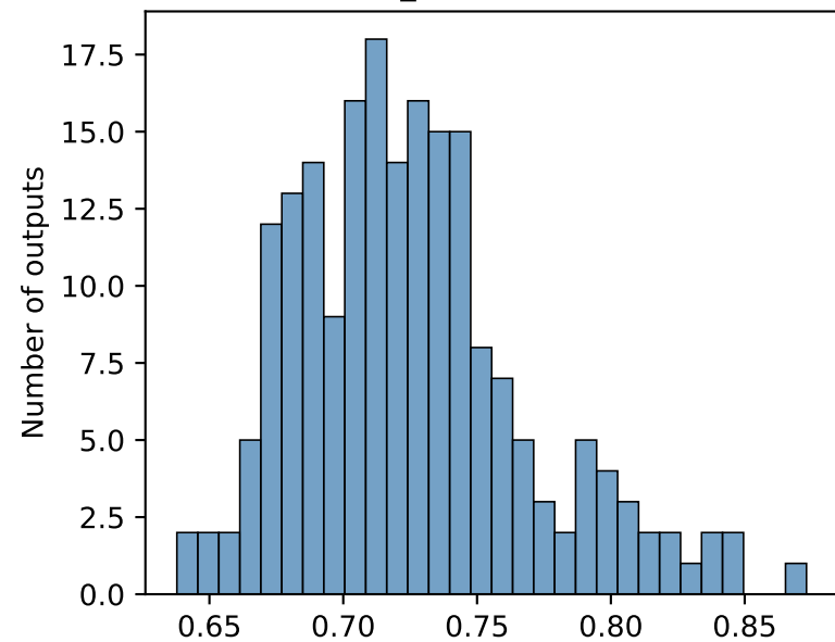
Flatness_mean distribution
