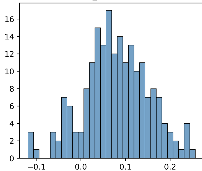
Flux_std distribution
