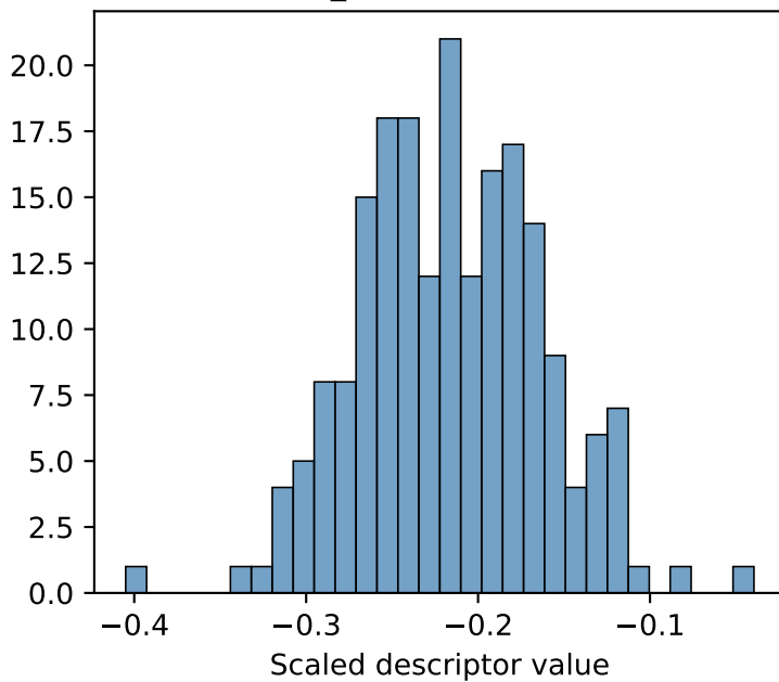
Flux_std distribution
