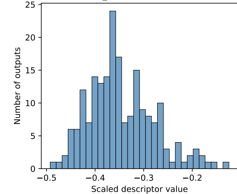
Flux_mean distribution
