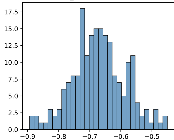
Flux_skewness distribution
