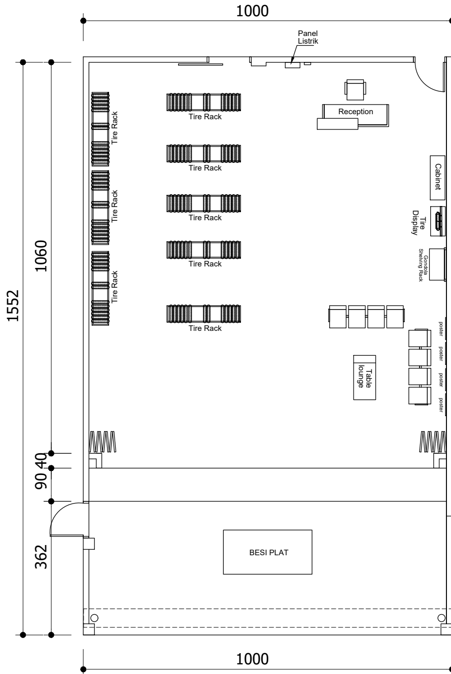
DENAH LAYOUT ARIES MOTOR
