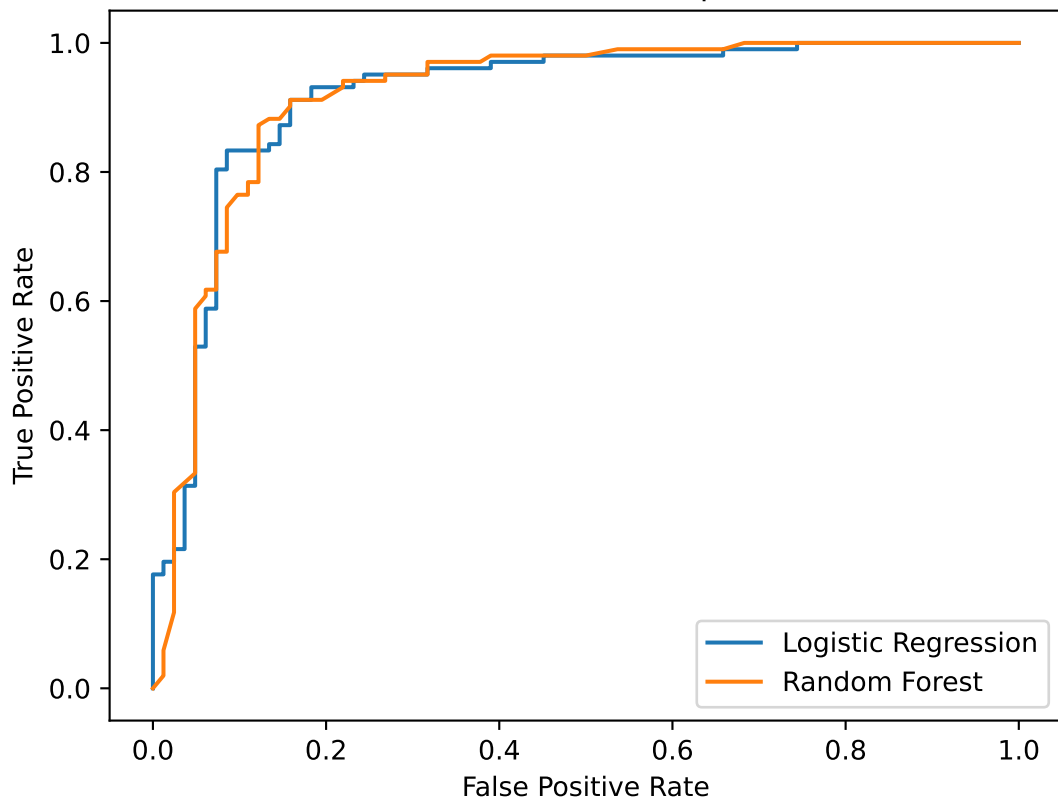
RQ2: ROC Curve Comparison
