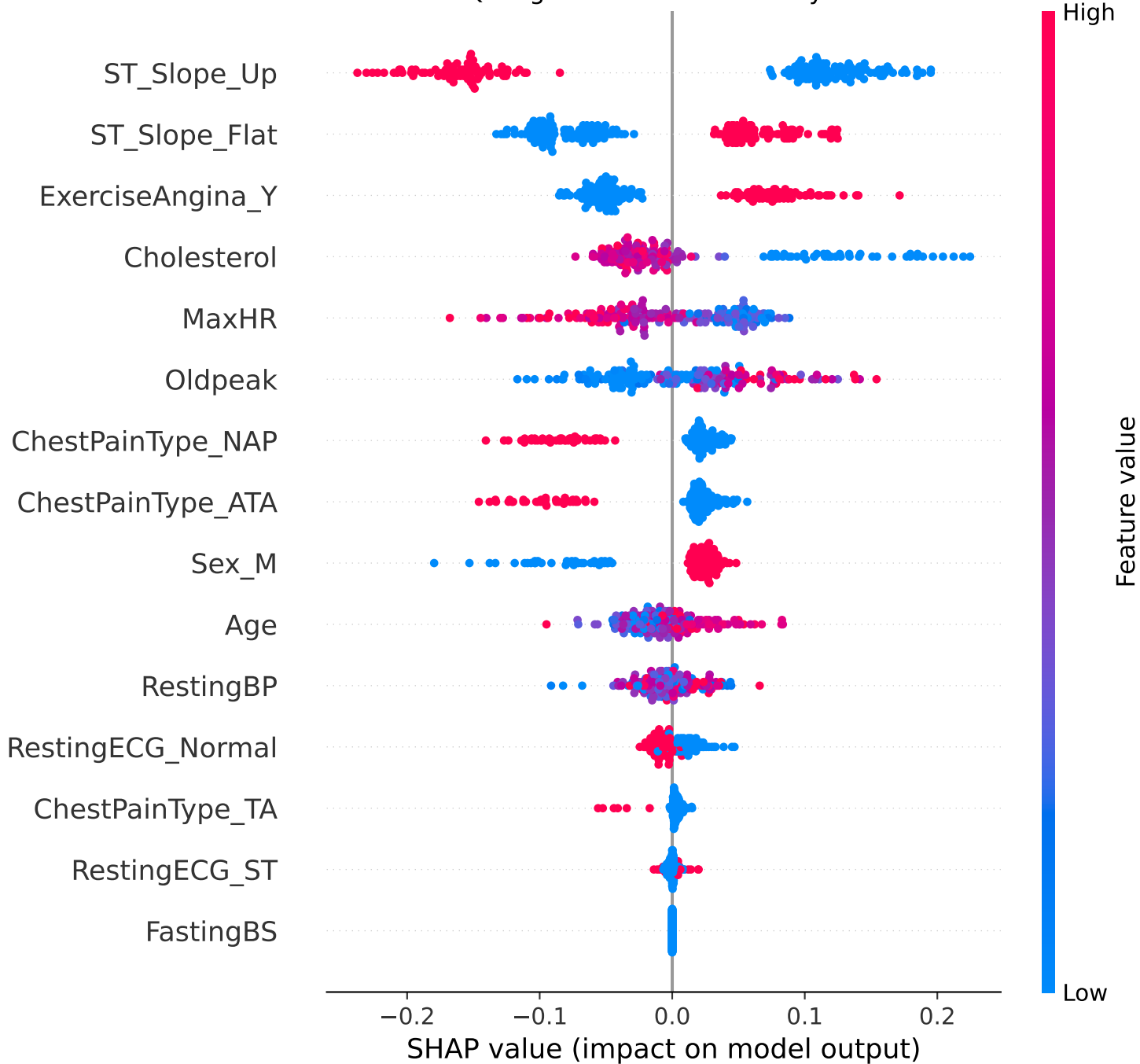
RQ3 Figure 7: SHAP Summary Plot
