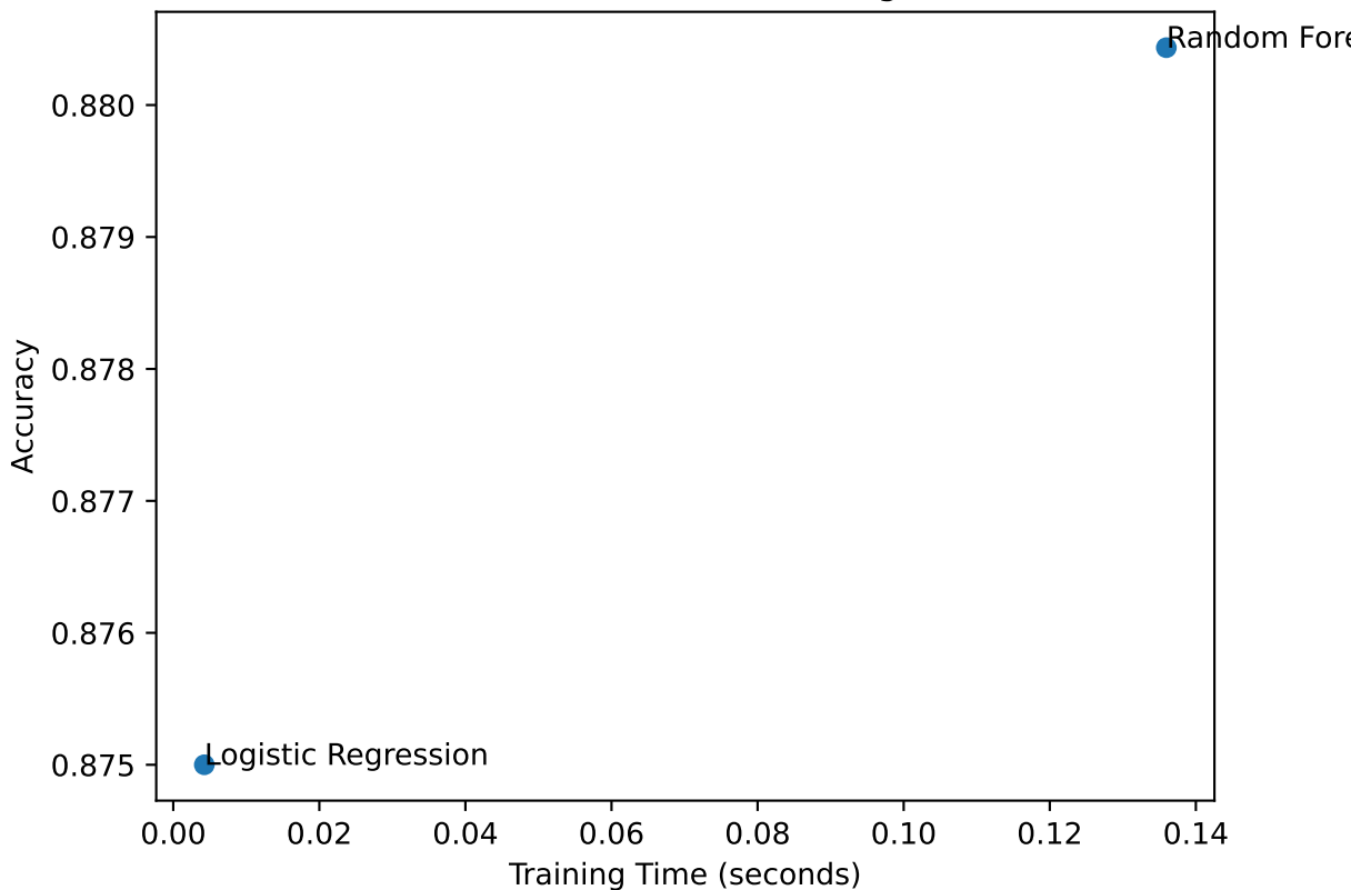
RQ2: Performance vs Training Time
