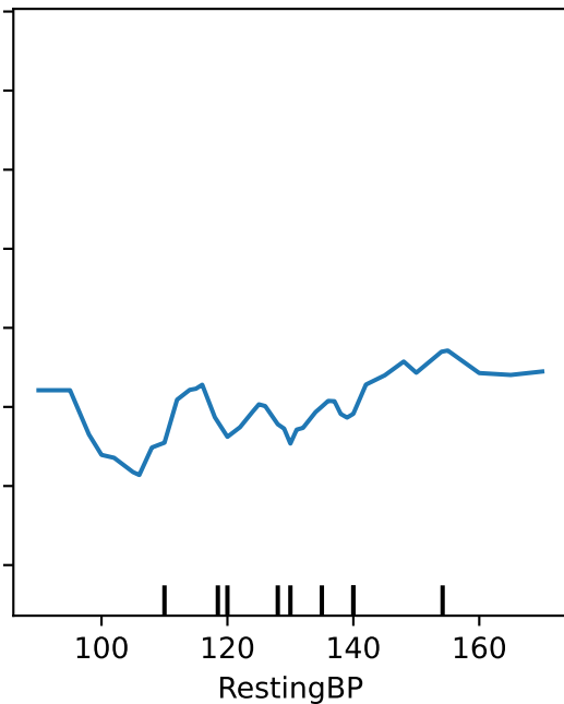
RQ3 Figure 9: Partial Dependence Plots
