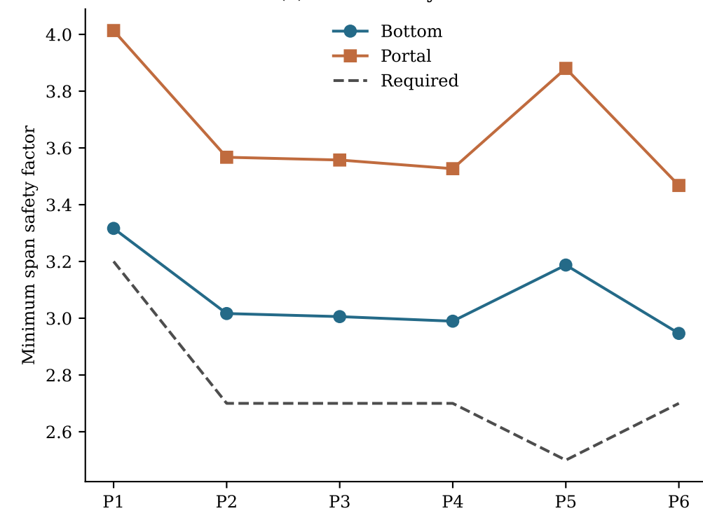
(c) Cable safety factors
