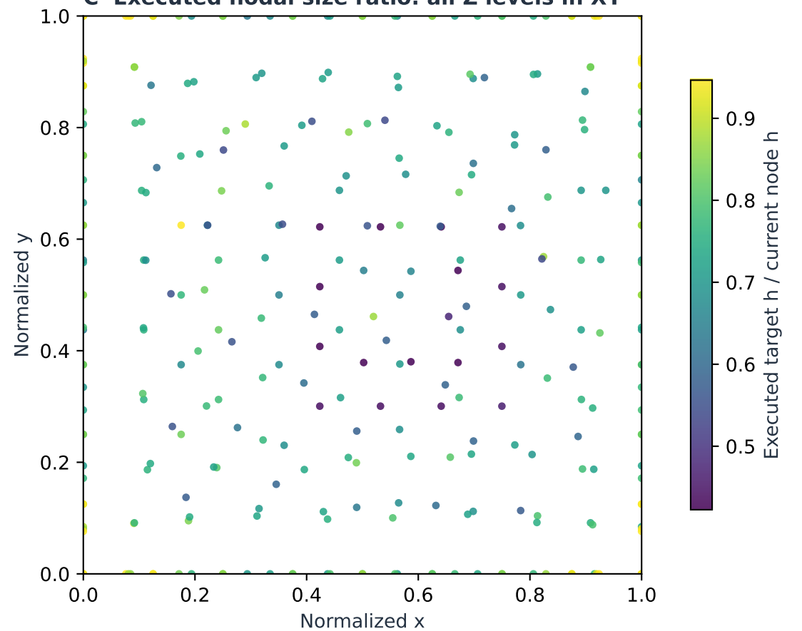
C Executed nodal size ratio: all Z levels in XY
