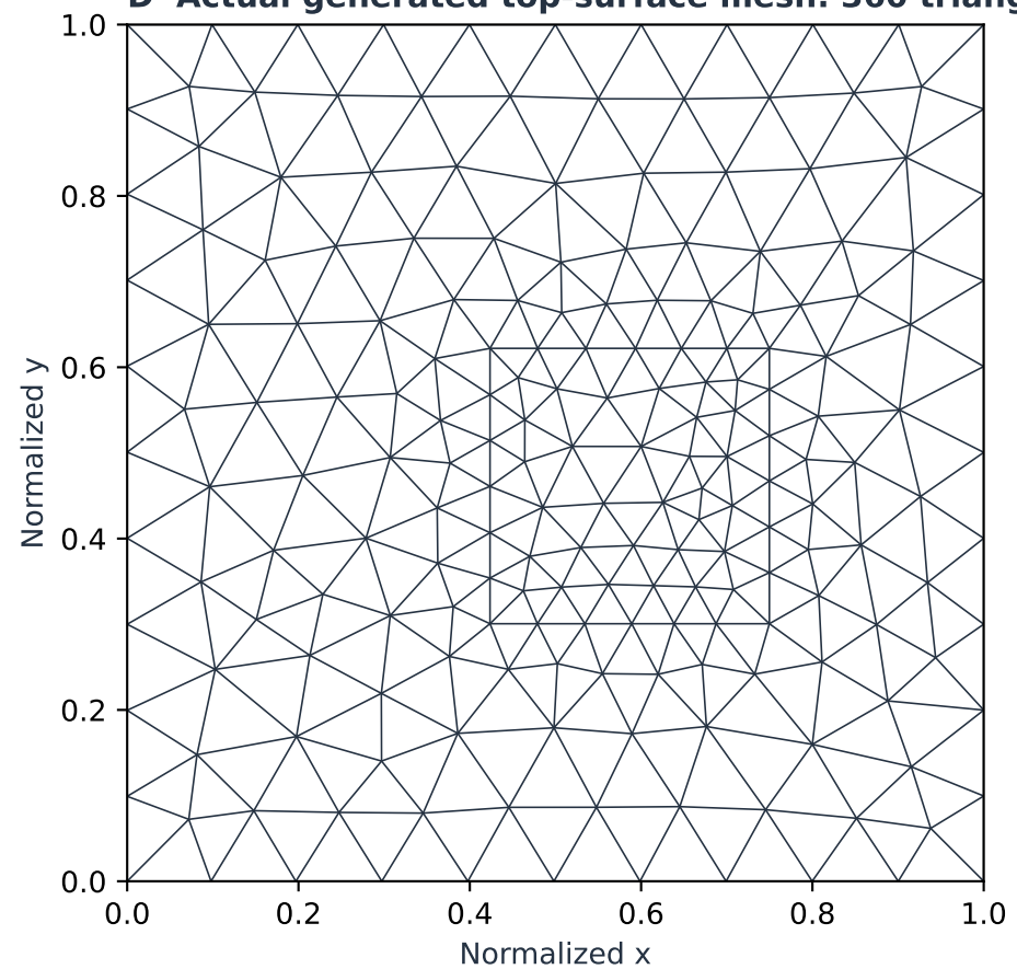
D Actual generated top-surface mesh: 360 triangles
