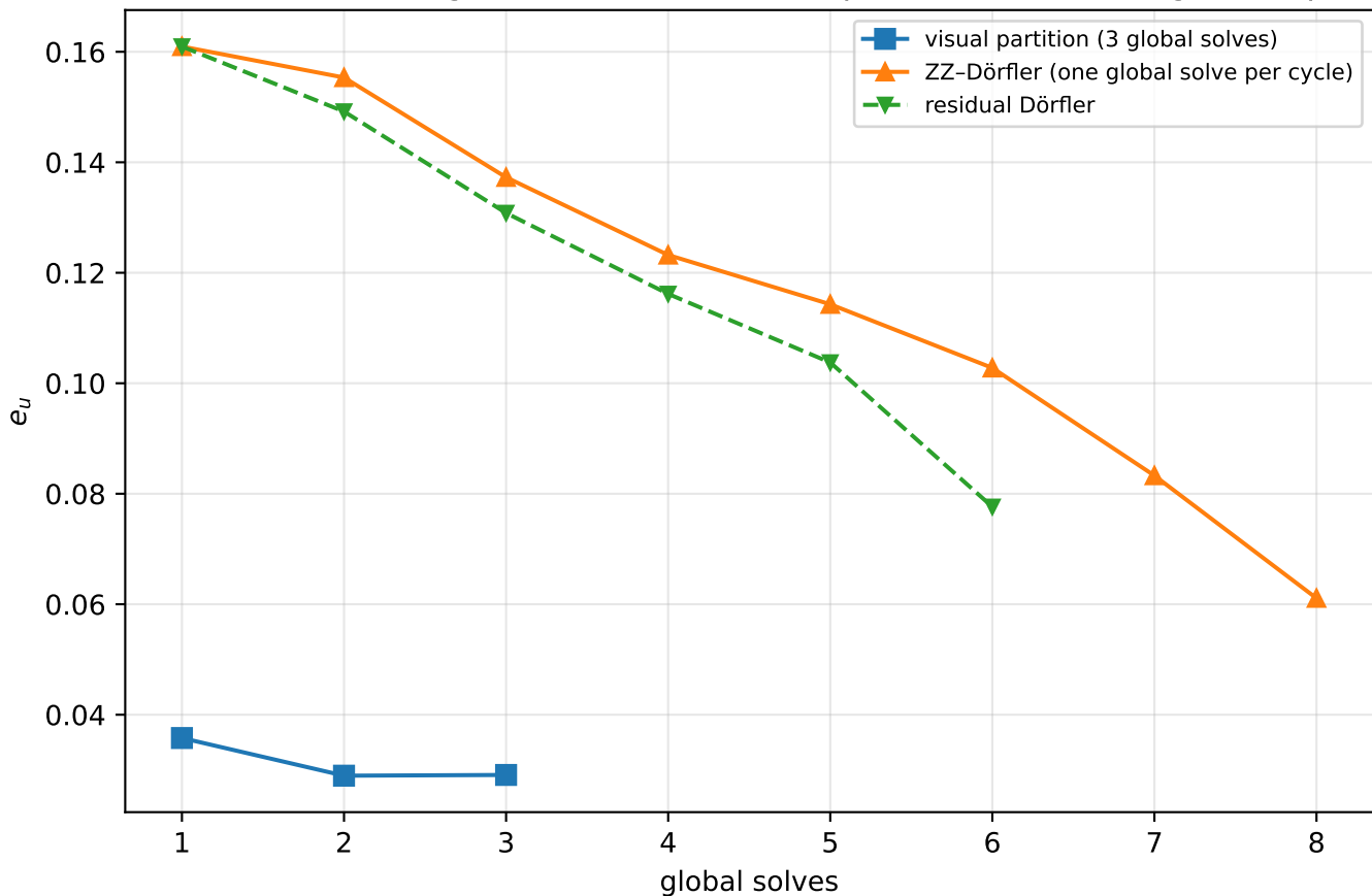
G01 S-LIN vs number of global solves. Dörfler is per-element marking, not a partition
