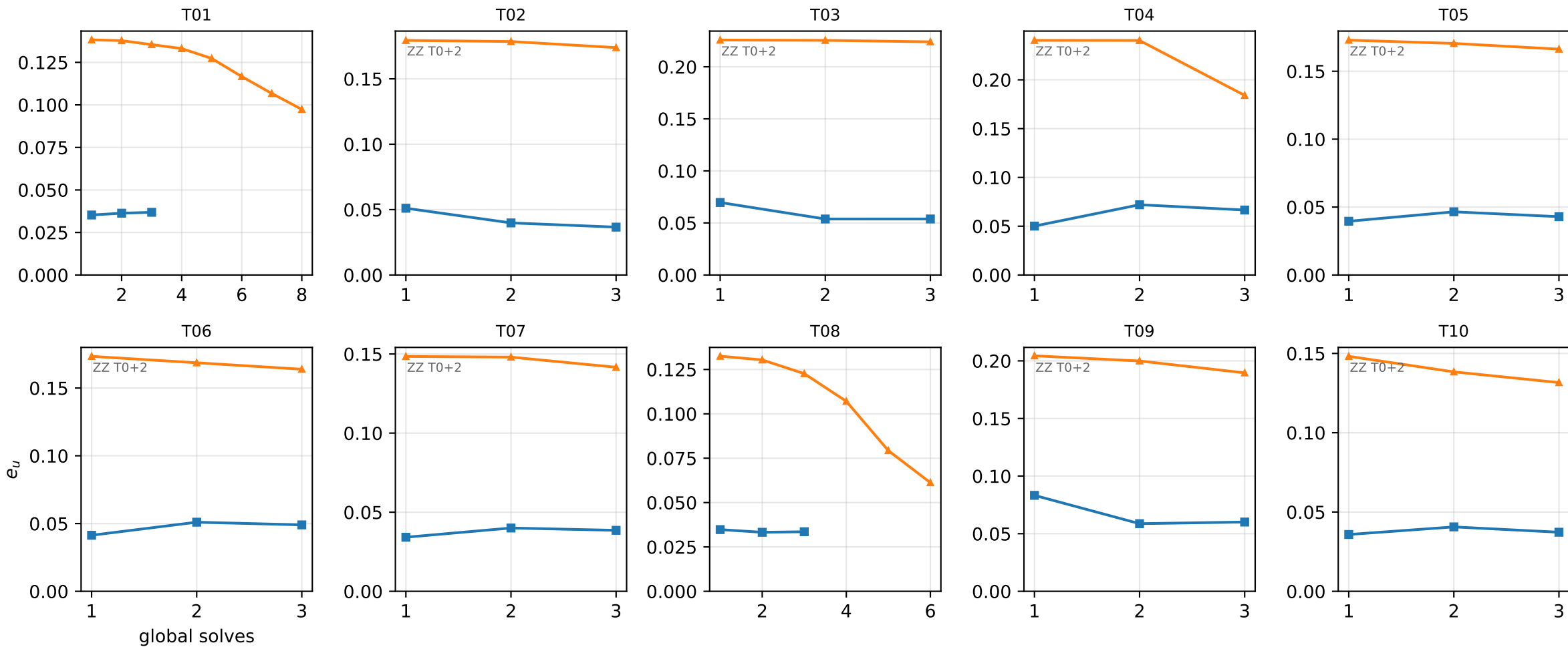
Ten tapers, S-LIN. Blue squares: visual partition. Orange triangles: hanging ZZ-Dörfler.
