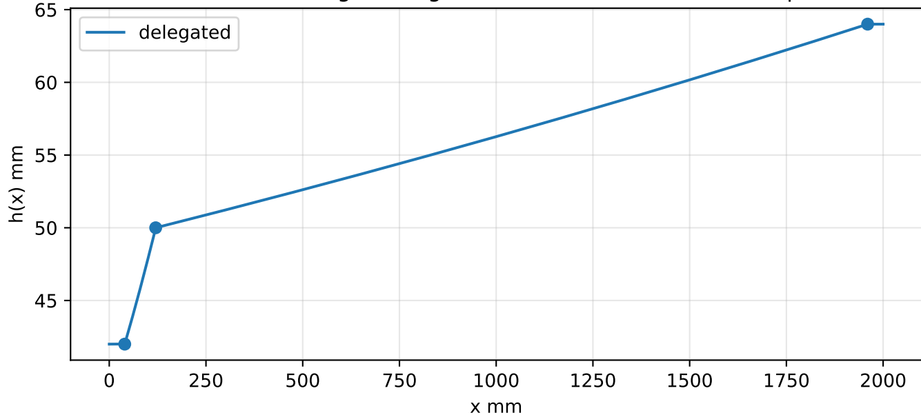
G01 S-LIN delegated log-linear size field. Not X0-X5 steps.
