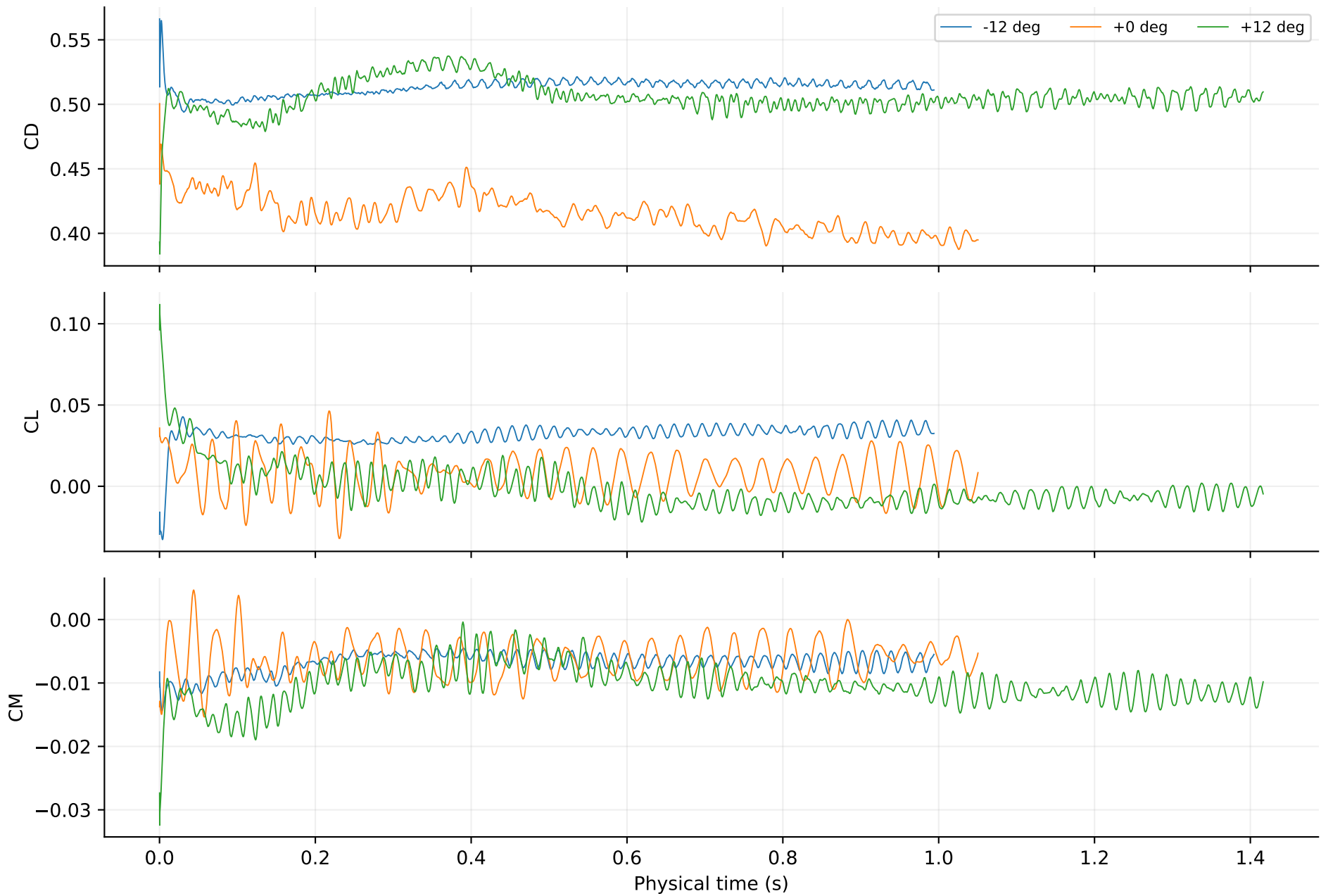
Native OpenFOAM coefficient histories
