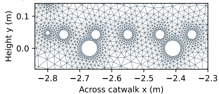
Original Gmsh mesh near side screen and carrier ropes
