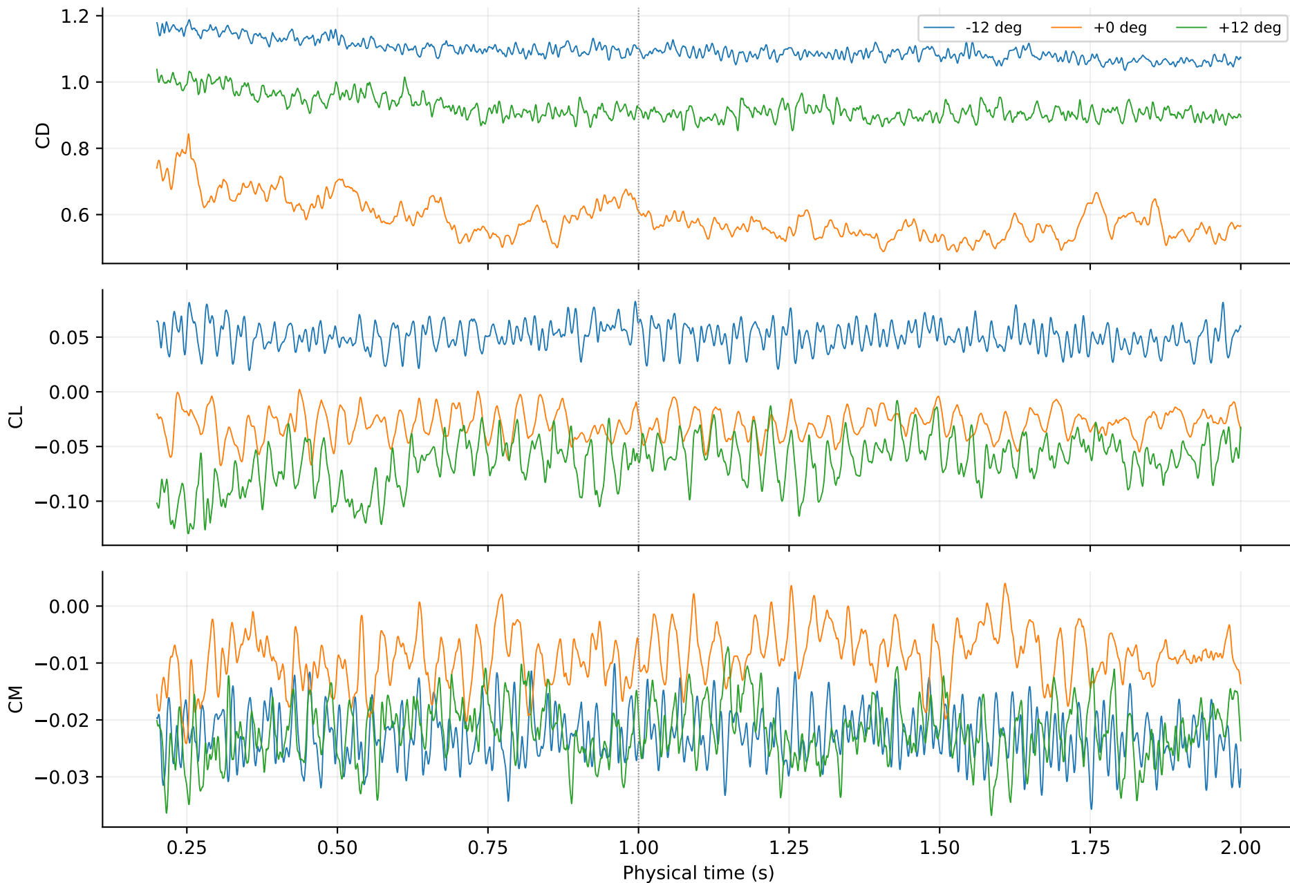
Native OpenFOAM histories; initial transient omitted from plot, complete samples in CSV
