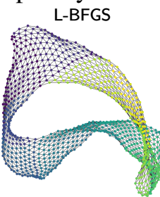
dwt_1005 ( |V| = 1005, |E| = 3808 , sparsity = 0.755%) Figures are at 100 iterations.
