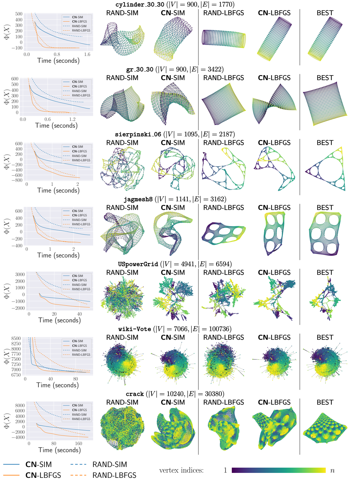
Figure 13: Additional experimental results for the FR force model. The objective function values at early states are generally improved for both simulation-based and L-BFGS algorithms, and the visual improvements by our proposed method CN are apparent for the simulation-based algorithms. The BEST column shows the reference layout obtained by running CN-LBFGS for 1000 iterations.
