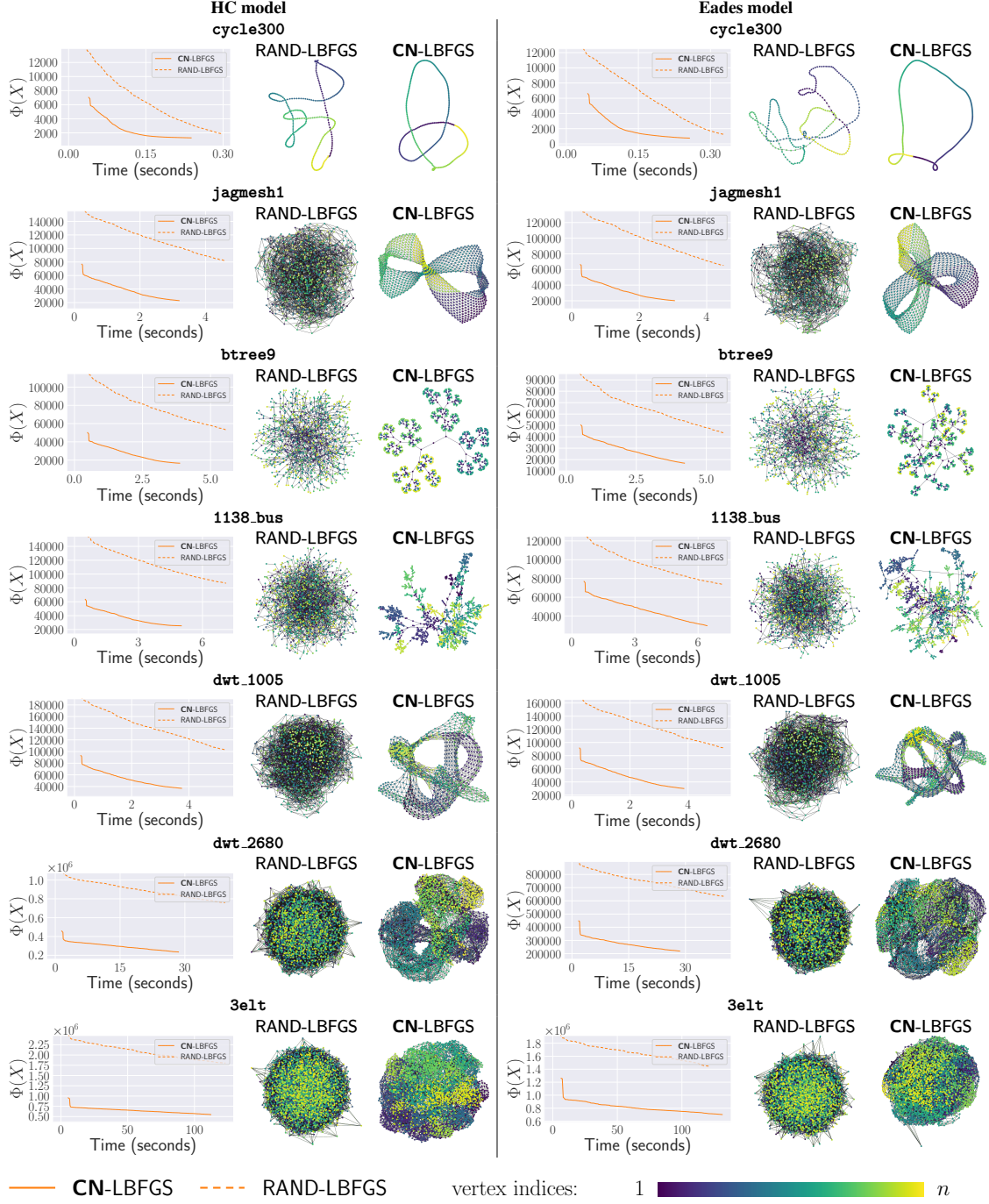
Figure 7: Experimental results for the HC and Eades force models. Our proposed method CN yields improved results.
