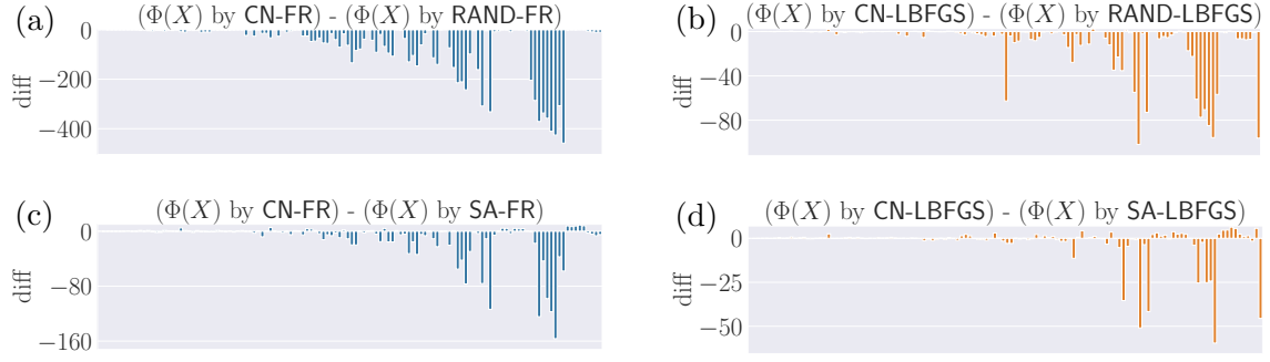
Figure 8: Comparison of the initializations. The bins arranged along the x-axis correspond to the 124 graphs. The y-axis shows the difference in \Phi(X) between CN and the baseline initialization method, averaged over ten trials. Panels (a) and (b) compare CN with RAND, whereas panels (c) and (d) compare CN with SA. Blue ones show results obtained using SIM, whereas orange ones show results obtained using LBFGS. In almost all cases for RAND and in most cases for SA, the differences are negative, meaning that the proposed initialization produced better final layouts than the baseline initialization methods.
