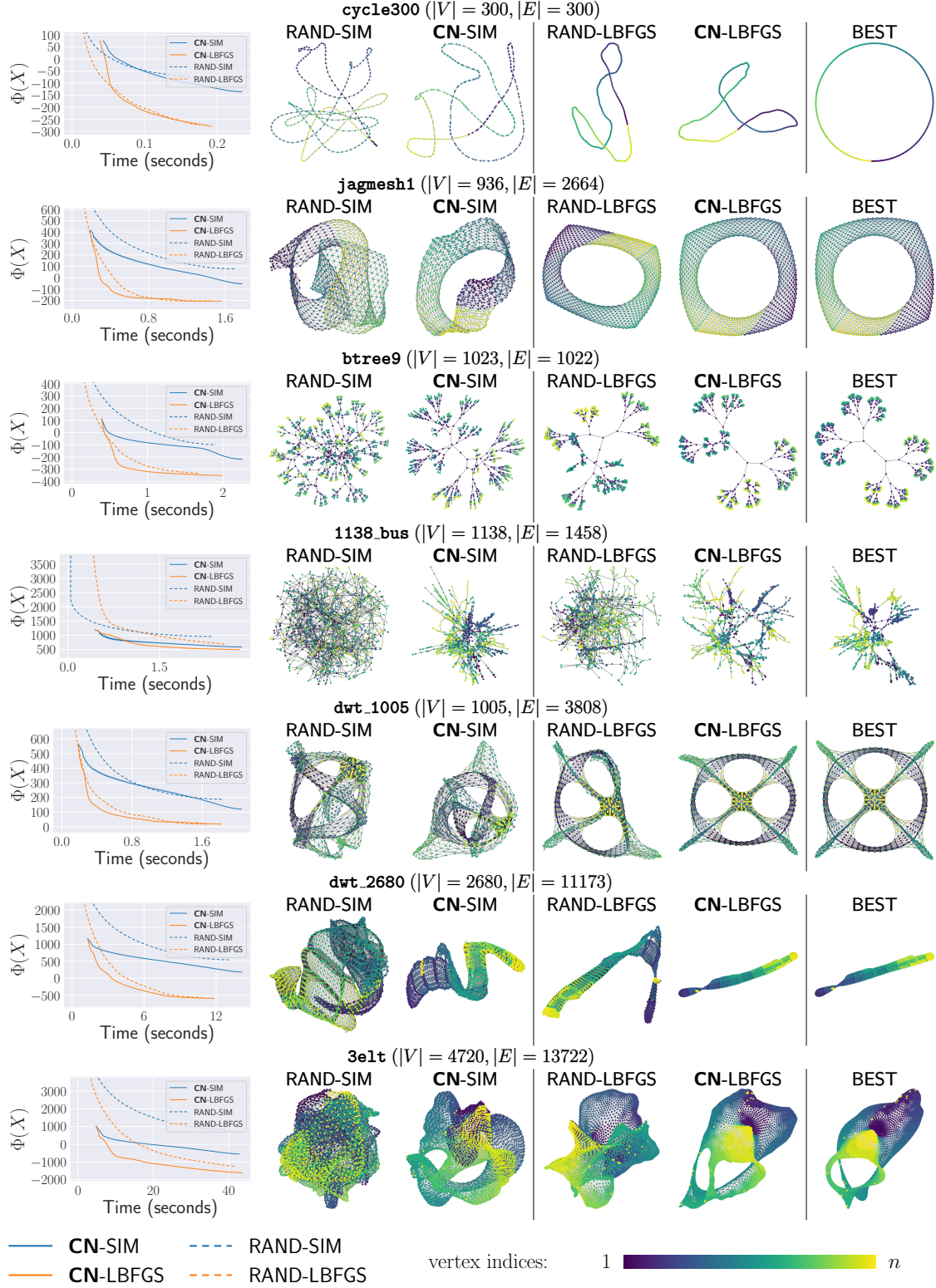
Figure 6: Experimental results for the FR force model. Our proposed method CN yields improved results for both the simulation-based algorithm and L-BFGS. The BEST column shows the reference layout obtained by running CN-LBFGS for 1000 iterations.
