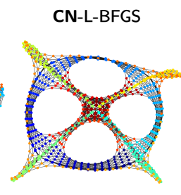
btrees9 ( |V| = 1023, |E| = 1022 , sparsity = 0.196%) Figures are at 150 iterations.
