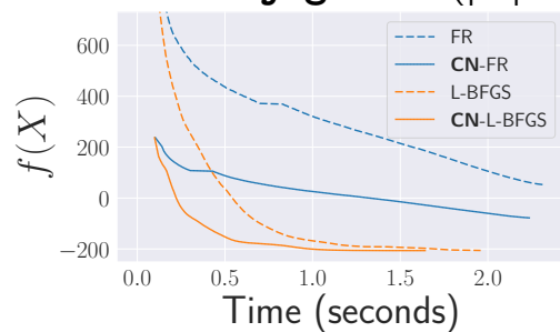
dwt_1005 ( |V| = 1005, |E| = 3808 , sparsity = 0.755%) Figures are at 100 iterations.
