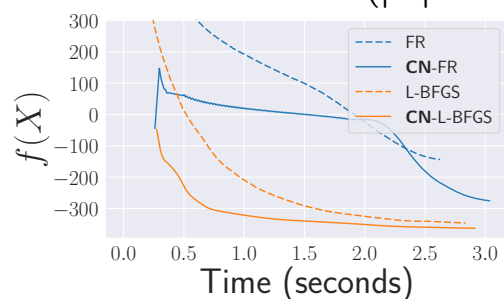
1138_bus ( |V| = 1138, |E| = 1458 , sparsity = 0.225%) Figures are at 150 iterations.
