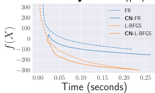
jagmesh1 ( |V| = 936, |E| = 2664 , sparsity = 0.609%) Figures are at 50 iterations.
