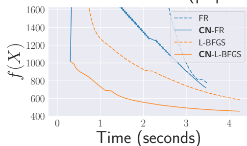
dwt_2680 ( |V| = 2680, |E| = 11173 , sparsity = 0.311%) Figures are at 150 iterations.
